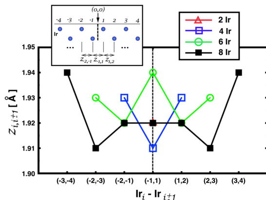
Figure 1. Out-of-plane distances between different Ir planes for ... Fe/ n_{\text{Ir}} Ir/Fe ... [ n_{\text{Ir}} = 2, 4, 6, 8 ] geometries. The center of each configuration has been shifted to the vertical dashed line that represents the central out-of-plane distance for any configuration. The x -axis values depict each Ir layer pair, i and i \pm 1 .
