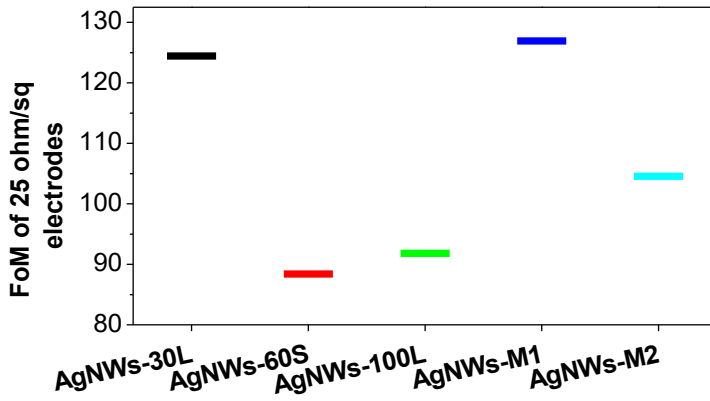
Fig.4 Figure of merit (FoM) of various silver nanowires electrodes with sheet resistance of 25 \Omega \text{ sq}^{-1} .
