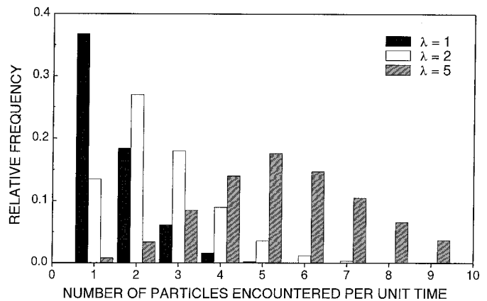
Fig. 8. Probability distributions of a Poisson variable for encounter rates ( \lambda ) of 1, 2, and 5. Note that the unit of time for the x-axis scale is arbitrary.
