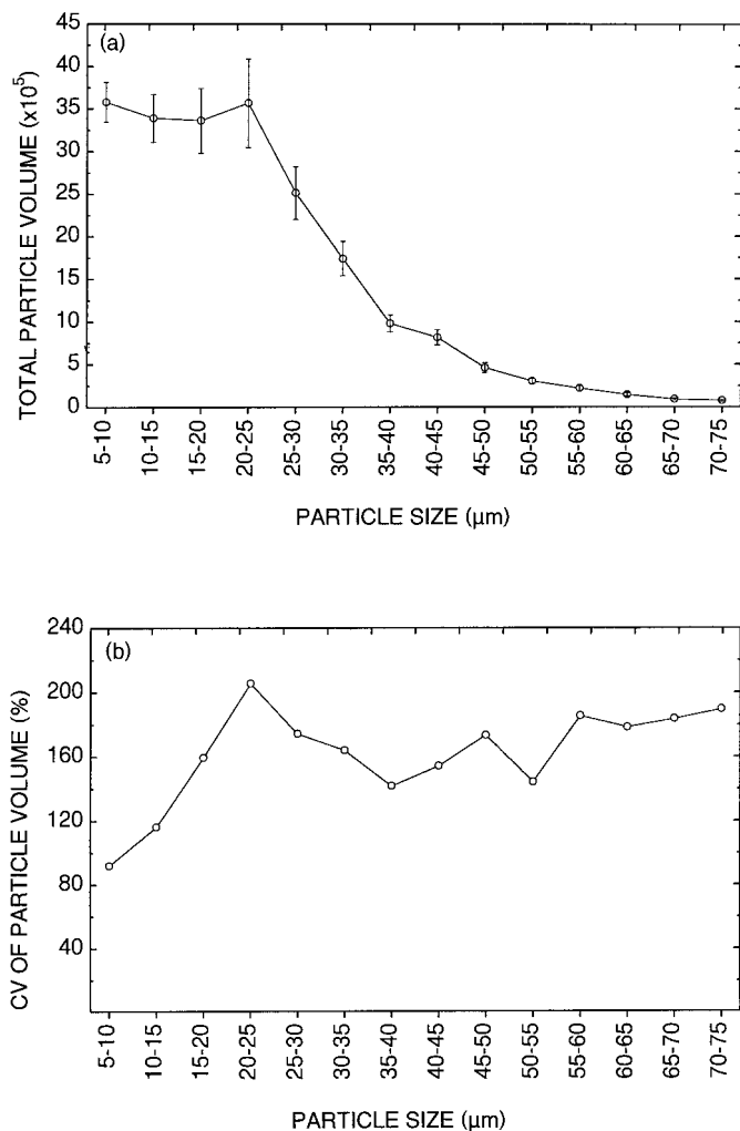
Fig. 7. (a) Mean ( \pm SE) of total particle volume (cubic micrometers) against particle size in 5- \mu m intervals, and (b) the C.V. of particle volume against particle size. Standard errors are shown in (a). The number of samples for each interval is 168.
