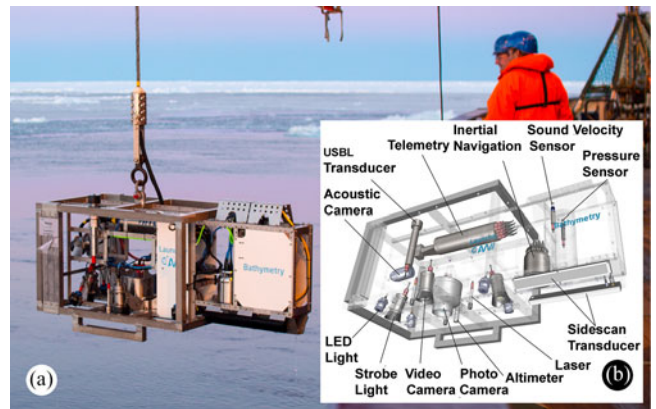
Fig. 1. OFOBS subsea unit. (a) Photographed during PS101 deployment during icy conditions. PHOTO: Frederic Tardeck, FIELAX. (b) Schematic of subsea unit.
