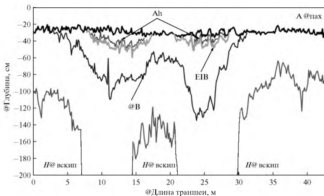
Fig. 1. Morphological structure of the trench in the year 2000. The designations: (Ah) the second humus horizon forming typical "microlows" in the paleorelief within the soil body; ( H @ \text{вскип} ) the effervescence depth upon treating the soil with a 10% HCl solution
