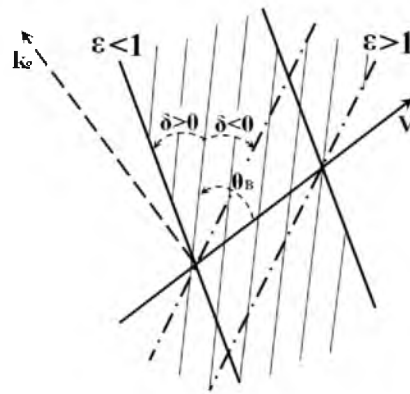
Fig. 2 Asymmetric ( \epsilon > 1, \epsilon < 1 ) reflections of radiation from a crystal plate.
