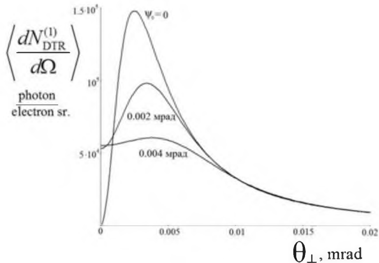
Fig. 6 The same, that in Fig. 4 under value of relativistic electron energy E = 200\Gamma\vartheta B .
