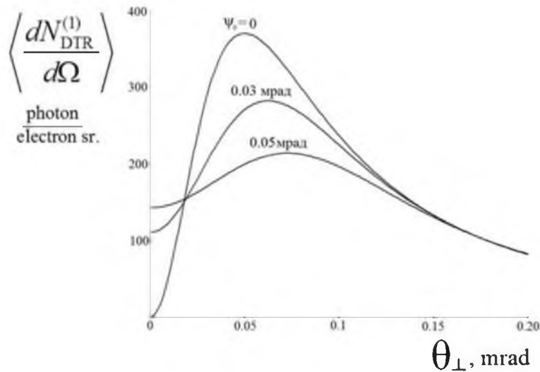
Fig. 5 The same, that in Fig. 4 under value of relativistic electron energy E = 10\Gamma\vartheta B .
