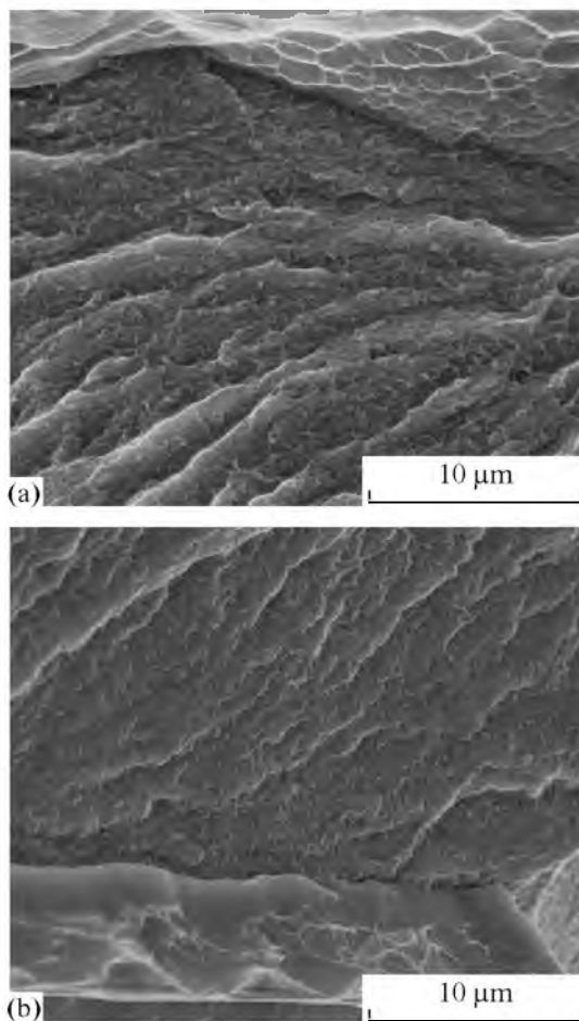
Fig. 5. Microstructure of the alloy samples annealed at (a) 350 and (b) 400°C.
