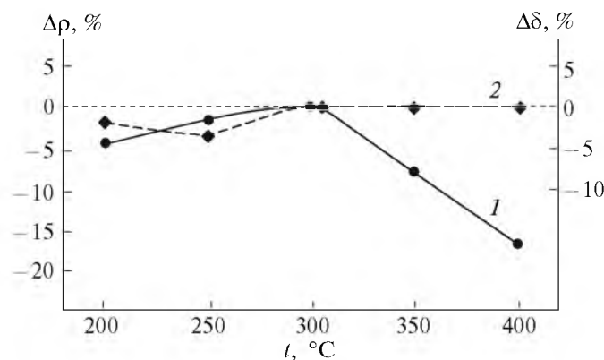
Fig. 1. Dependences of (1) the relative change on electrical resistivity, \Delta\rho , and (2) the thickness \Delta\delta of amorphous alloy samples on the annealing temperature.
