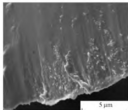
Fig. 3. Nano- and microcrystals at the surface of an amorphous ribbon annealed at 300°C.
