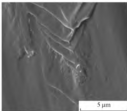
Fig. 4. Nanocrystals in the region deformed as a result of the alloy sample breaking in liquid nitrogen after annealing at 300°C.
