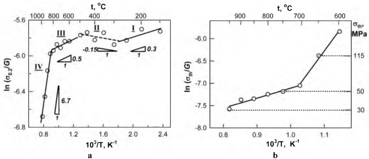
Figure 4. (a) Yield stress \sigma_{0.2} and (b) “threshold” stress \sigma_{th} normalized by the shear modulus G(T) as functions of the reciprocal deformation temperature.
