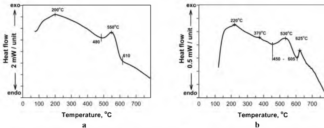
Figure 1. DSC thermogram of Ni-20%Cr alloy heated at 20°C/min (a) in the water quenched condition after solution treatment at 1100°C, (b) and after severe cold deformation by a Bridgman anvil to a strain of ~6.
