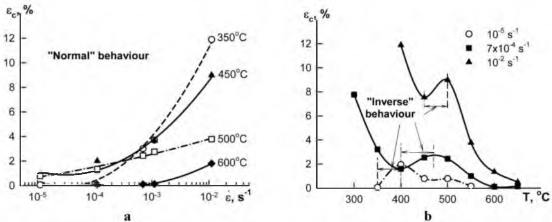
Figure 3. Variation of the critical strains with strain rate (a) and temperature (b) of deformation.
