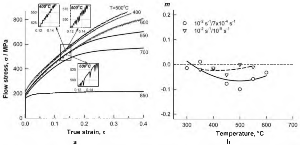
Figure 2. (a) True stress – true strain curves at temperatures of 400-850°C and strain rate of 7 \times 10^{-1} \text{ s}^{-1} and (b) temperature dependence of the coefficient, m , of strain-rate sensitivity of the flow stress.
