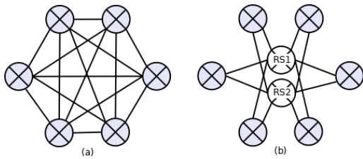
Fig. 1. Bi-lateral (a) vs Multi-lateral (b) peering for a full-mesh connection between 6 ASes. In bi-lateral peering n \cdot (n - 1)/2 BGP sessions would be required. MLP would require only n sessions with the Route Server, or 2n when two Route Servers are used for redundancy.
