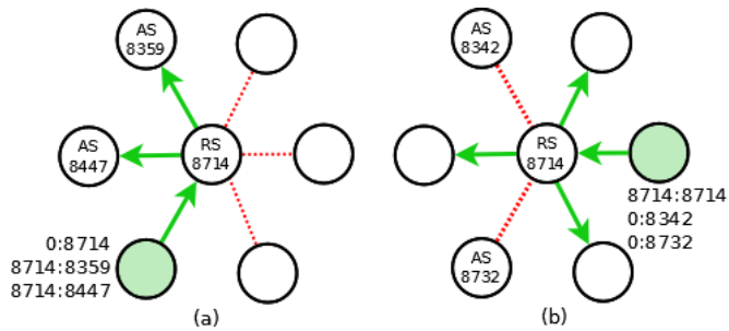
Fig. 2. Control of route advertisements in a Route Server using BGP Communities
