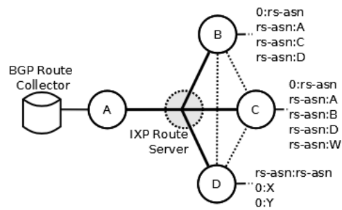
Fig. 3. Discovery of missing Route Server peerings through the use of BGP Communities.
