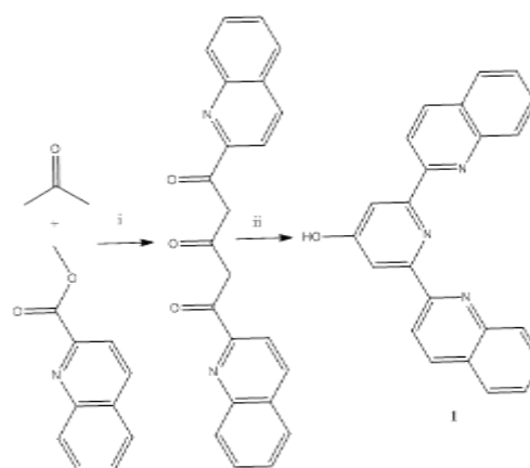
Scheme 1. Synthesis of 2,6-bis(2-quinolyl)-4(1H)-pyridone 1 . i) NaOBu t , THF 60°C 16h; ii) NH 4 OAc, MeOH, 60°C, 16h.
