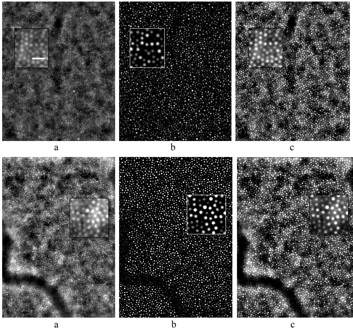
Figure 5.10: Image enhancement with the Hessian-LoG filter. (a) Processed retinal image; (b) Hessian-LoG filtered image; (c) image (a) multiplied with image (b). The scale bar is 21 \mu\text{m} .
