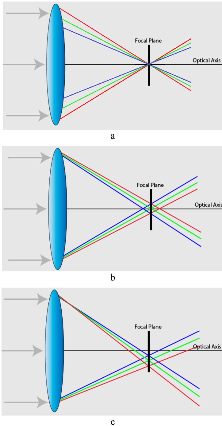
Figure 1.8: Schematic drawing showing (a) a perfect lens with no chromatic aberration, (b) longitudinal chromatic aberration and (c) transverse chromatic aberration [37].
