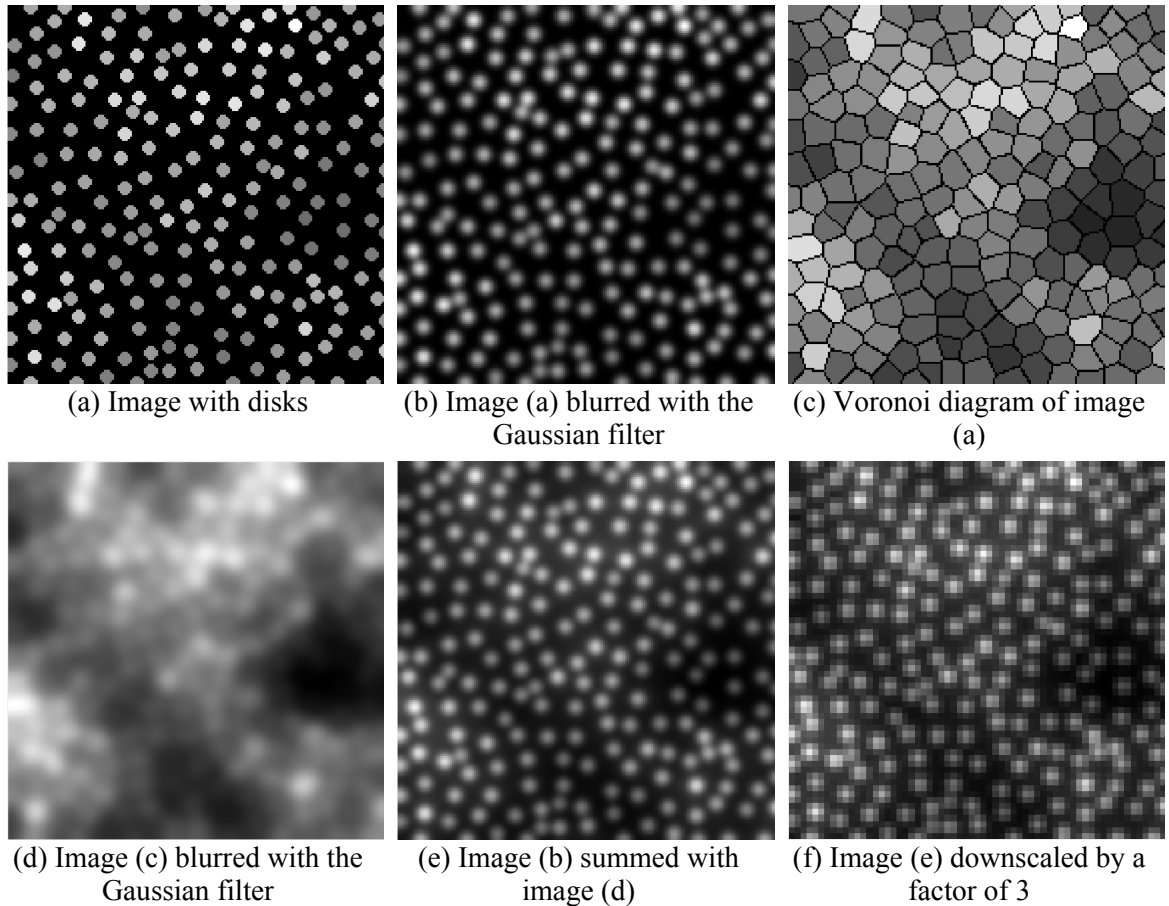
Figure 4.6: Step-by-step process of synthetic image generation.
