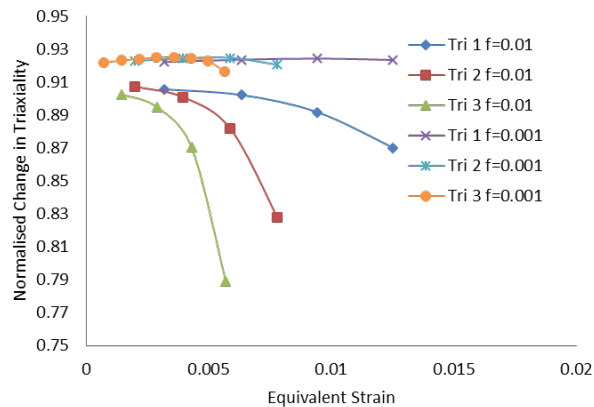
Figure 6: Normalised change in volume averaged triaxiality for two different porosities and 3 different applied triaxialities
