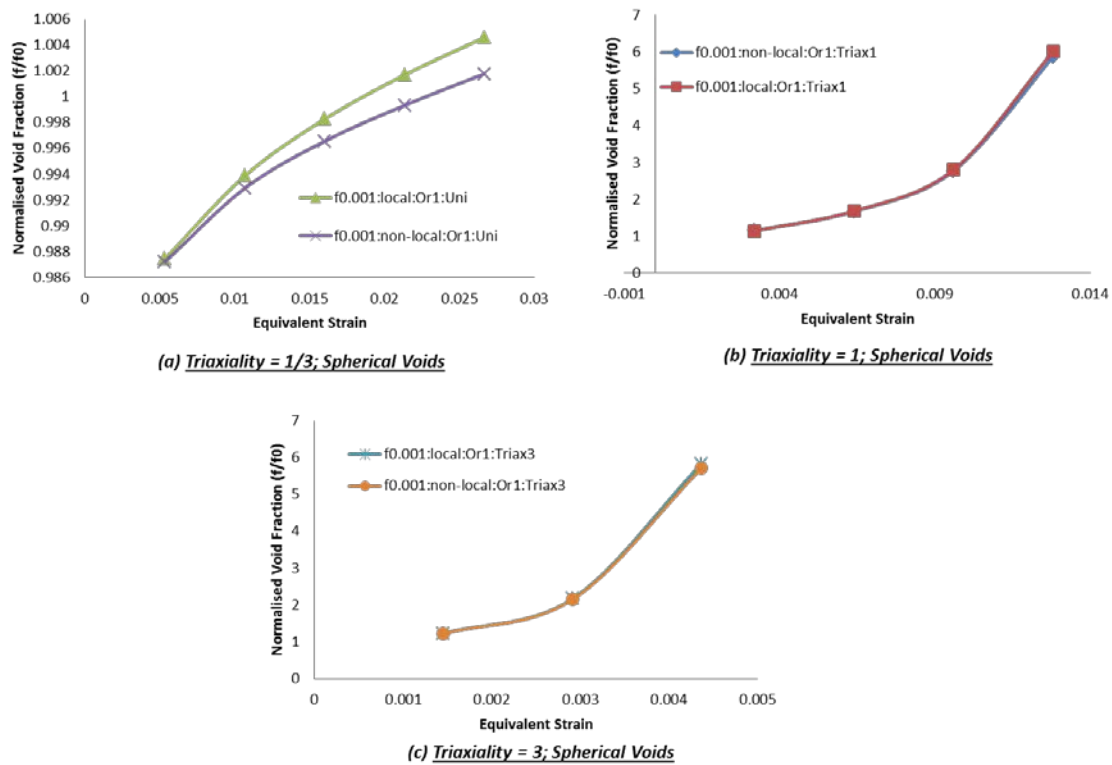
Figure 9: Effect of Strain gradients on void growth for void size = 800 \mu\text{m}
