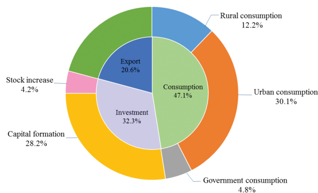
Figure 4. Compositions of embodied emission by Chinese economy.
