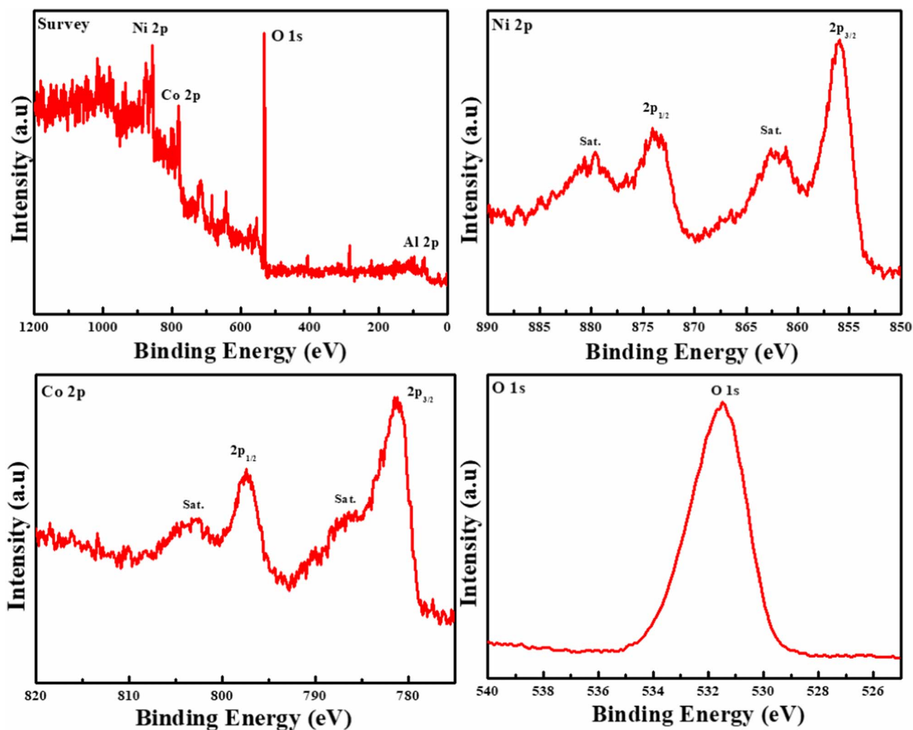
Figure 4. XPS spectra of the sample: (a) the survey spectra, (b)-(d) core level spectra of the Ni 2p, Co 2p and O 1s region, respectively.
