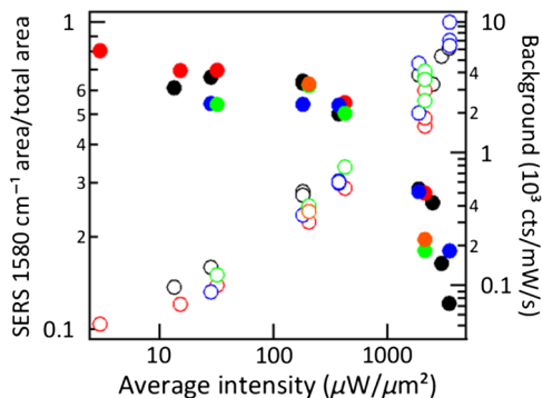
FIG. 11. Extracted relative intensity of the 1580-cm -1 Raman mode detected from five individual NPoM (solid dots, left axis) and SERS background extracted at 2000 cm -1 (open dots, right axis), as a function of increasing CW laser power. Points of different color correspond to different nanoparticles.
