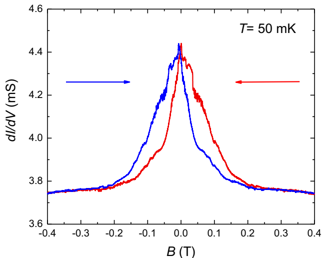
Fig. 3. Magnetoconductance oscillations and hysteresis on the differential conductance of the Nb-In 0.75 Ga 0.25 As-Nb Josephson junction: Differential conductance ( dl/dV ) vs. applied magnetic field B perpendicular to the junction's plane at temperature 50 mK. Arrows indicate the B sweep directions.
