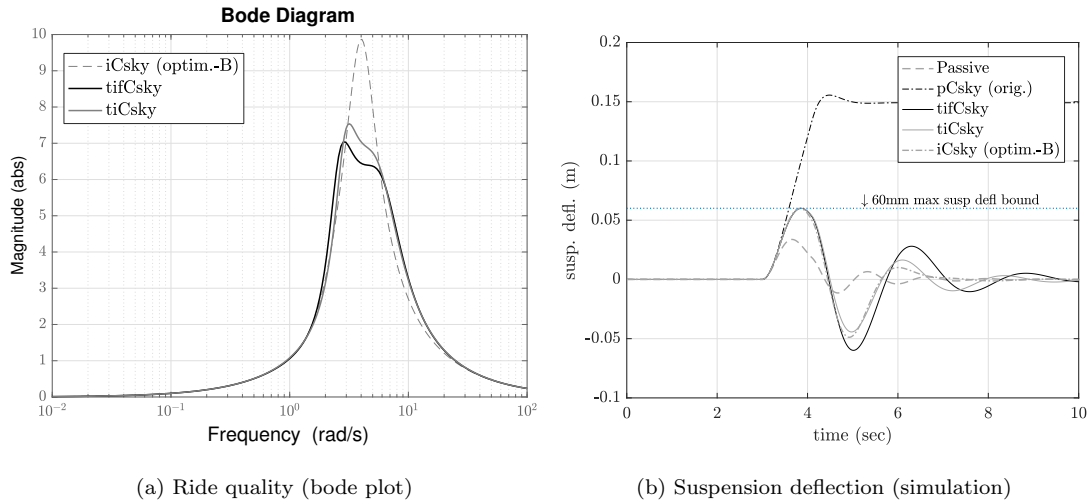
Figure 14. Fractional order skyhook performance
