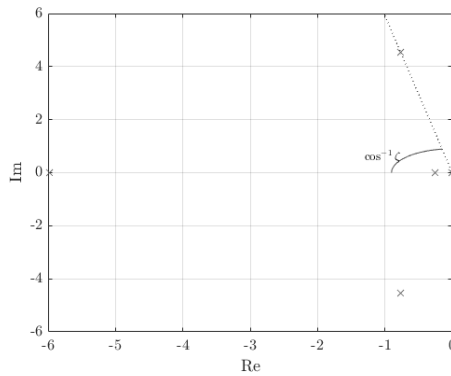
(c) Poles location in s -plane (rational)
