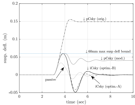
Figure 4. Suspension deflection conventional skyhook damping schemes (deterministic)
