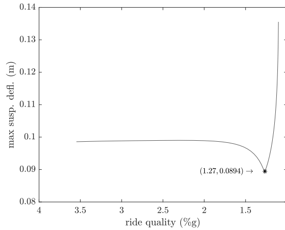
Figure 3. Deterministic/ Stochastic trade-off for iCsky (man.) (2nd order L_{HP} )
