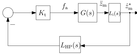
Figure 2. Feedback setup for implemented skyhook scheme
