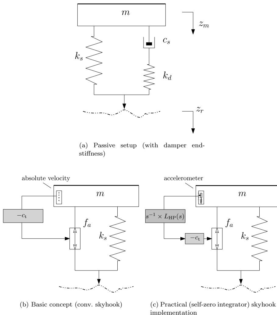
Figure 1. Passive and skyhook damping control schemes
