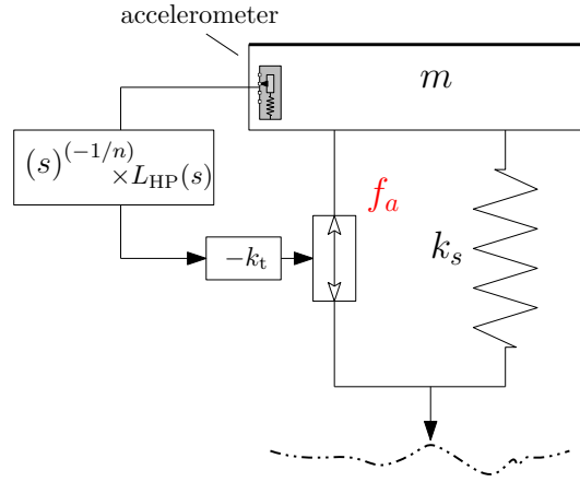
Figure 7. Practical skyhook damping scheme with fractional order (tilted) integrator
