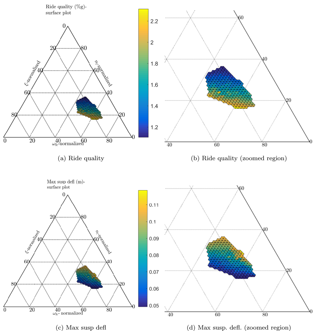
Figure 13. Ternary diagram surface plots for tifCsky
