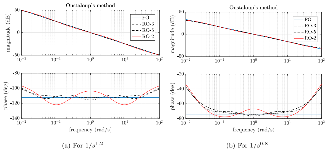
Figure 6. Fractional order integration and rational approximation examples (Bode plot)
