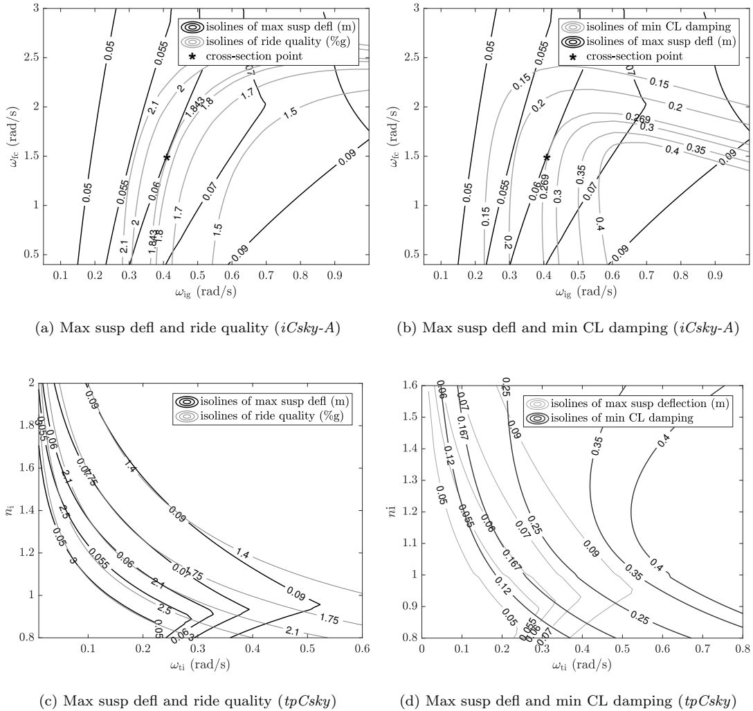
Figure 5. Contour lines for optimised iCsky (optim.-A) and optimised tpCsky
