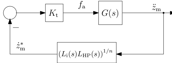
Figure 12. Skyhook feedback control scheme with FO “self-zero” integrator ( tifCsky )
