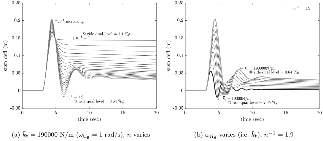
Figure 8. Effect of fractional integration on pCsky (fractional system simulation)
