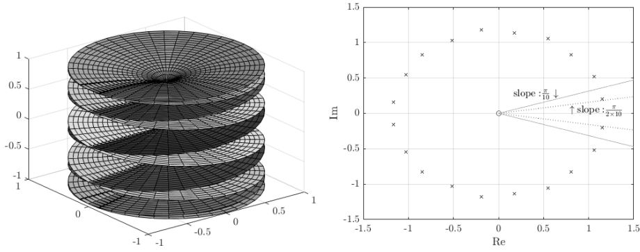
(a) Riemann surface of w = s^{\frac{1}{10}} (10-sheets) (b) Poles location in w -plane (fractional)
