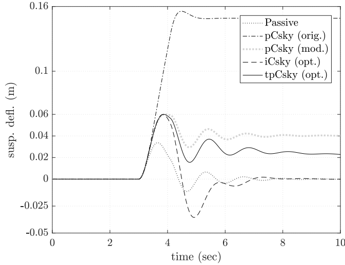
Figure 9. Suspension deflection response for tpCsky vs conv. skyhook schemes
