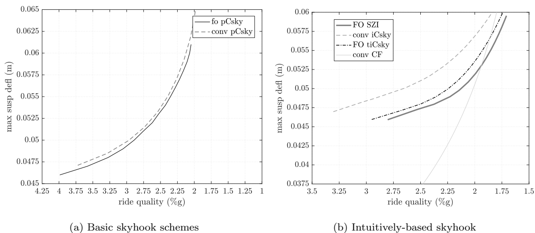
Figure 10. Ride quality (rq)/ max susp deflection (msd) trend (best rq per msd)
