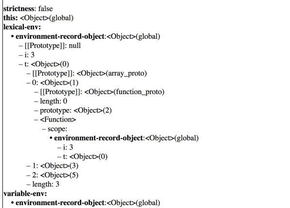
Figure 12: Display of the state and environment of the interpreted code. The environment includes the local variables.
