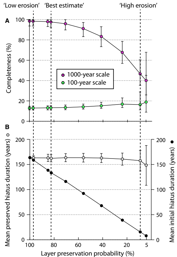
Fig. 6. (A) Summary of completeness statistics for model scenarios with varying layer preservation probability that reproduce a ca 75 cm Grey Shales Member-like succession of 220 ± 10 layers deposited in 36 000 years. Note how completeness at the 1000 year scale is sensitive to layer preservation probability, but that completeness at the 100 year scale is largely invariant to changing layer preservation probability. See main text for details. (B) Mean preserved hiatus durations and mean initial hiatus durations. Note how the mean preserved hiatus duration does not vary significantly with layer preservation probability. The mean initial hiatus duration (i.e. the mean recurrence time between layer depositional events) falls with decreasing layer preservation probability. This reflects the fact that with higher erosion (i.e. decreased preservation probability) more layers need to be initially deposited to ensure preservation of ca 220 layers. All models use exponentially distributed erosion depths and hiatuses, and all results are based on analysis of 1000 simulations for each layer preservation probability scenario. Error bars show the 95% uncertainty.
