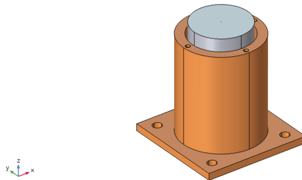
Figure 2. An interference fit monochromator design with copper sleeve as the hub component and single crystal silicon shaft as the shaft component.
