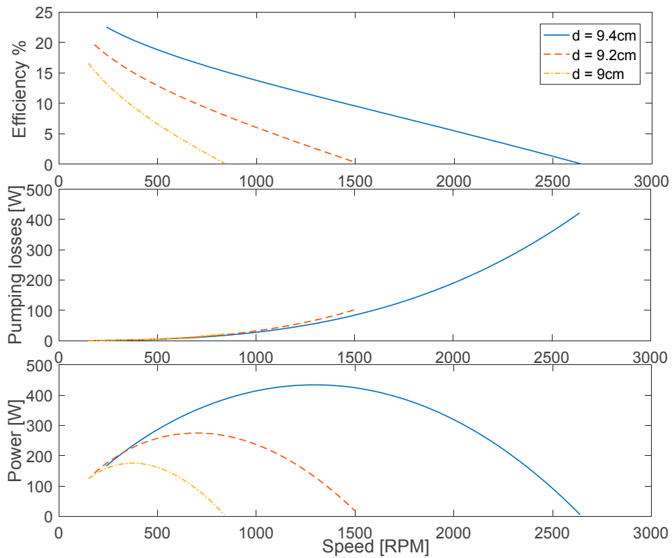
Figure 8. Influence of increasing the isothermal fins diameter on the Franchot engine performance for doubled Franchot engine cylinder diameter D_e = D_c = 10\text{ cm} .
