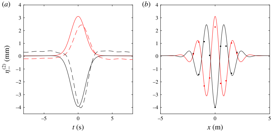
FIGURE 15. (Colour online) Temporal (a) and spatial (b) evolution of the wave-averaged surface elevation \eta_{-}^{(2)} at the focus point ( x = 0, y = 0 ) for two wave groups colliding head-on ( \Delta\theta = 180^\circ ). The red lines correspond to two groups that are in phase ( \mu_1 = \mu_2 ) and the black lines to groups that are out of phase ( \mu_1 - \mu_2 = 180^\circ ). The multiple-scale solution (2.15) is given by the continuous lines, and the measurements by the dashed lines in (a) and the dots in (b).
