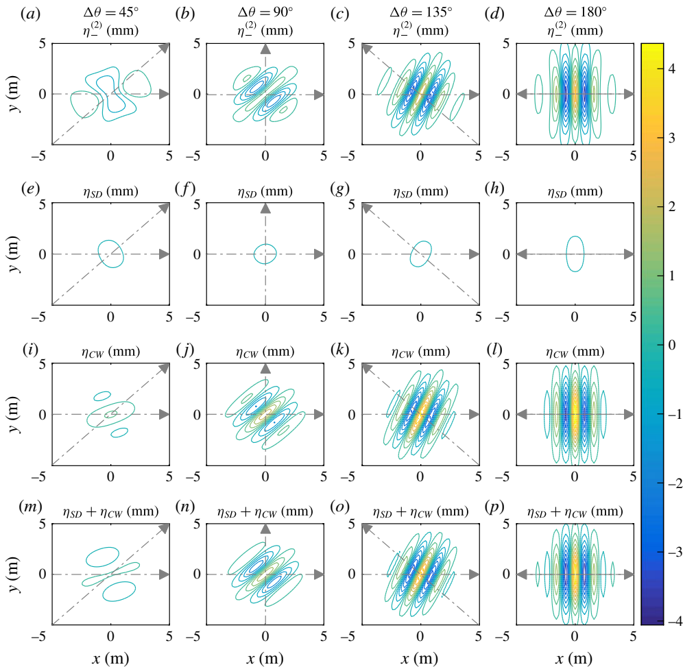
FIGURE 6. (Colour online) Contours of the wave-averaged surface elevation \eta_{-}^{(2)} for crossing wave groups at time of linear focus for different crossing angles \Delta\theta ; (a–d) are computed from multicomponent second-order theory (2.21), (e–h) correspond to the set-down in the quasimonochromatic limit (2.16)–(2.17), (i–l) correspond to the crossing wave pattern in the quasimonochromatic limit (2.19) and (m–p) correspond to the sum of the last two. The degree of spreading of the individual groups is \sigma_{\theta} = 10^{\circ} .
