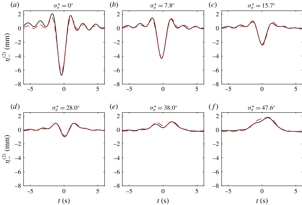
FIGURE 9. (Colour online) The wave-averaged surface elevation \eta_{-}^{(2)} at the central probe ( x = 0, y = 0 ) for the spreading tests (category A), showing measurements \eta_{M-}^{(2)} (black lines) and theoretical predictions \eta_{T-}^{(2)} (red dashed lines) for a linear input amplitude of a_0 = 0.15 m. The different panels correspond to increasing degree of input spreading \sigma_\theta = 0 – 50^\circ (see table 2) and the labels denote the estimated degree of spreading \sigma_\theta^* .
