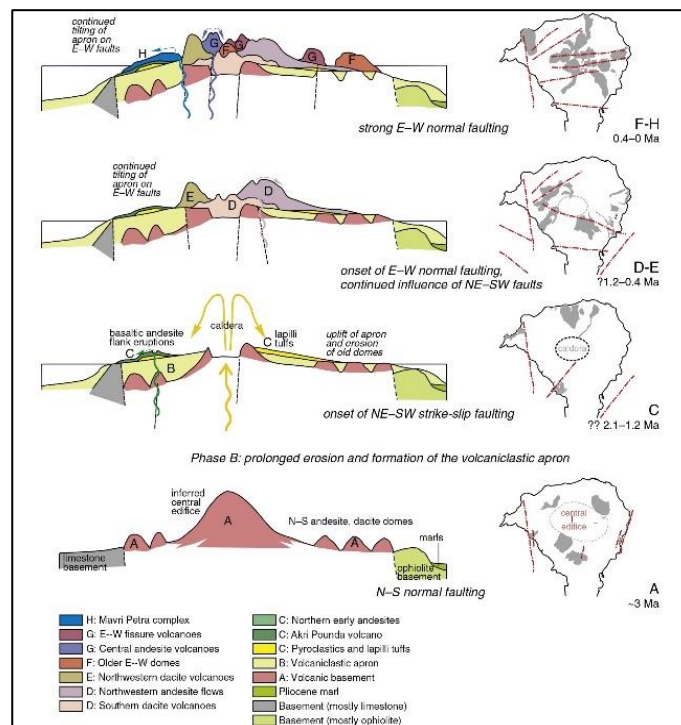
Figure 2: Schematic cross-sections (E-W or SE-NW) and maps of Methana, showing inferred relationship of volcanic stratigraphy to evolution of regional fault patterns. Cross sections illustrate stratigraphy; no representation of the magmatic plumbing system is attempted (Pe-Piper and Piper, 2013).
