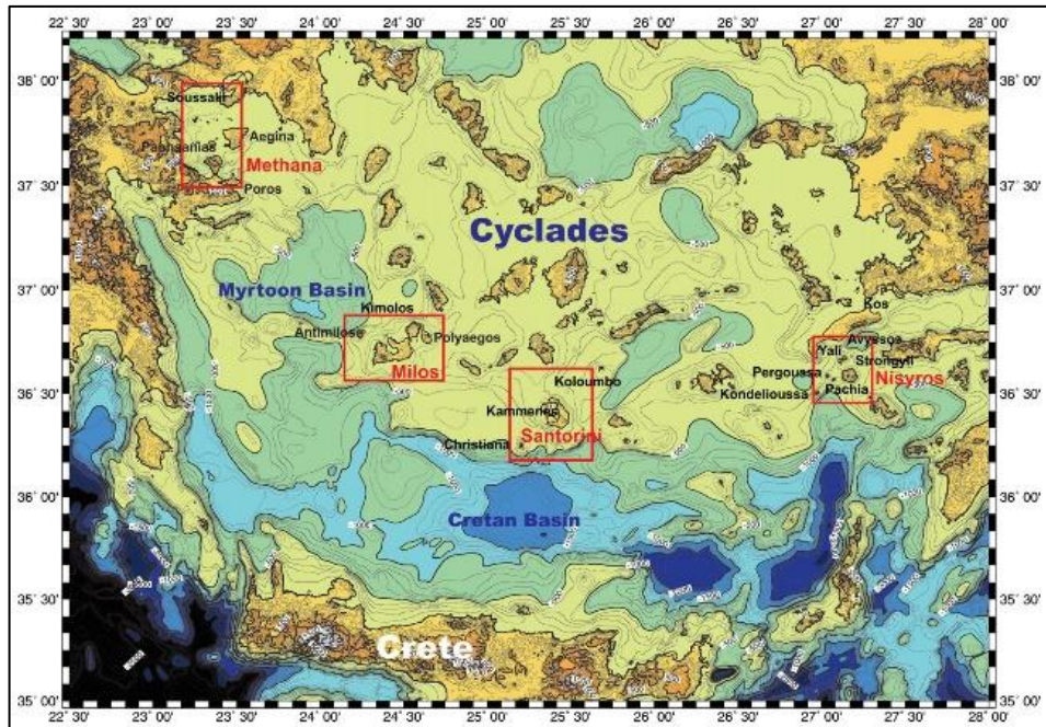
Figure 1: Topographic map of the southern Aegean Sea combining onshore and offshore data. The four modern volcanic groups are indicated within red boxes together with the names of the main terrestrial and submarine volcanic centers along the volcanic arc (Nomikou et al., 2013).
