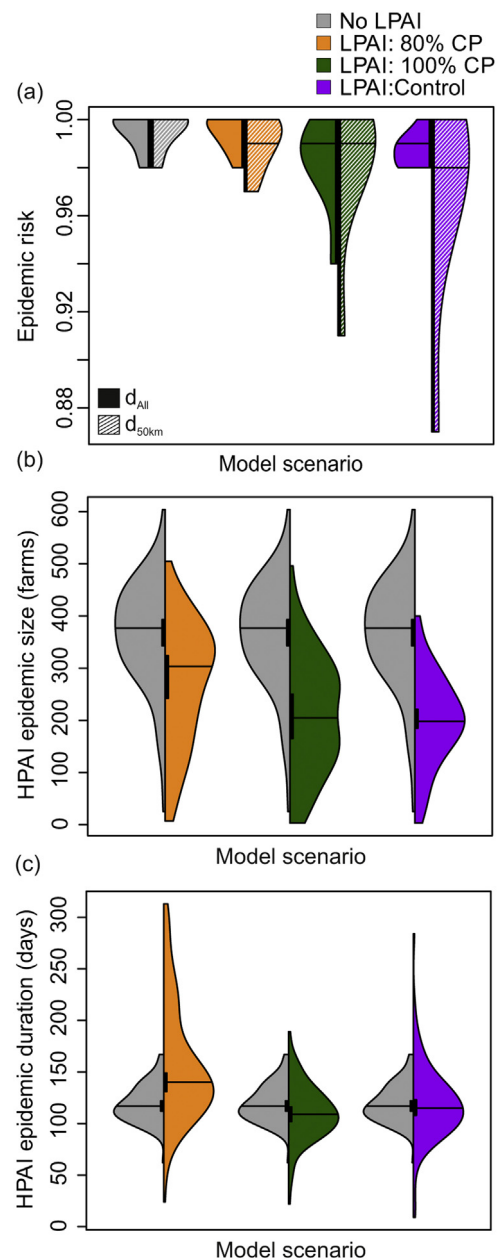
Fig. 4. Impact of immunological cross-protection and LPAI-targeted control on HPAI epidemic risk, size, and duration. Probability density function estimates based on spatial model simulations for (a) epidemic risk (probability of an HPAI epidemic i.e. > 10 cases). Each scenario is based on 100 \times 7 model simulations (100 simulations per LPAI prevalence investigated). Note decrease to lower limit of epidemic risk for 100% CP and LPAI-targeted control scenarios compared to in the absence of LPAI albeit with wide confidence intervals around the median estimate; (b) HPAI epidemic size; and (c) HPAI epidemic duration. Horizontal lines indicate median estimates and vertical bars indicate Binomial 95% confidence intervals around the median. For (a,c) each scenario is based on 100 model simulations and assumes a background LPAI prevalence of 6.2% ( n = 200 LPAI cases) upon HPAI emergence. Density plots were produced by adapting the ‘vioplot’ function of the package ‘violin’ available in R software v. 3.1.1 (Hintze and Nelson, 1998; R Core Team, 2013). See Supplementary material for sensitivity analysis.
