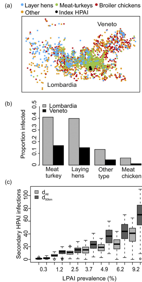
Fig. 3. Assessing the opportunity for epidemiological interference. (a) Spatial distribution of poultry farms located in Lombardia and Veneto, northeast Italy; (b) Region and production/species-specific incidence of HPAI infected farms; (c) Inter-quartile range of secondary HPAI infections across 100 model simulations for varying LP AI prevalence (corresponding with case numbers of 10, 40, 80, 120, 160, 200 and 300 infected farms) and distance to the 'emergent' HPAI-infected flock. d_{\text{All}} = no proximity constraint placed on location of LP AI cases; d_{50\text{km}} = LP AI cases constrained to within 50 km of the index HPAI farm. Note that these simulations were run in the absence of immunological cross-protection assumptions.
