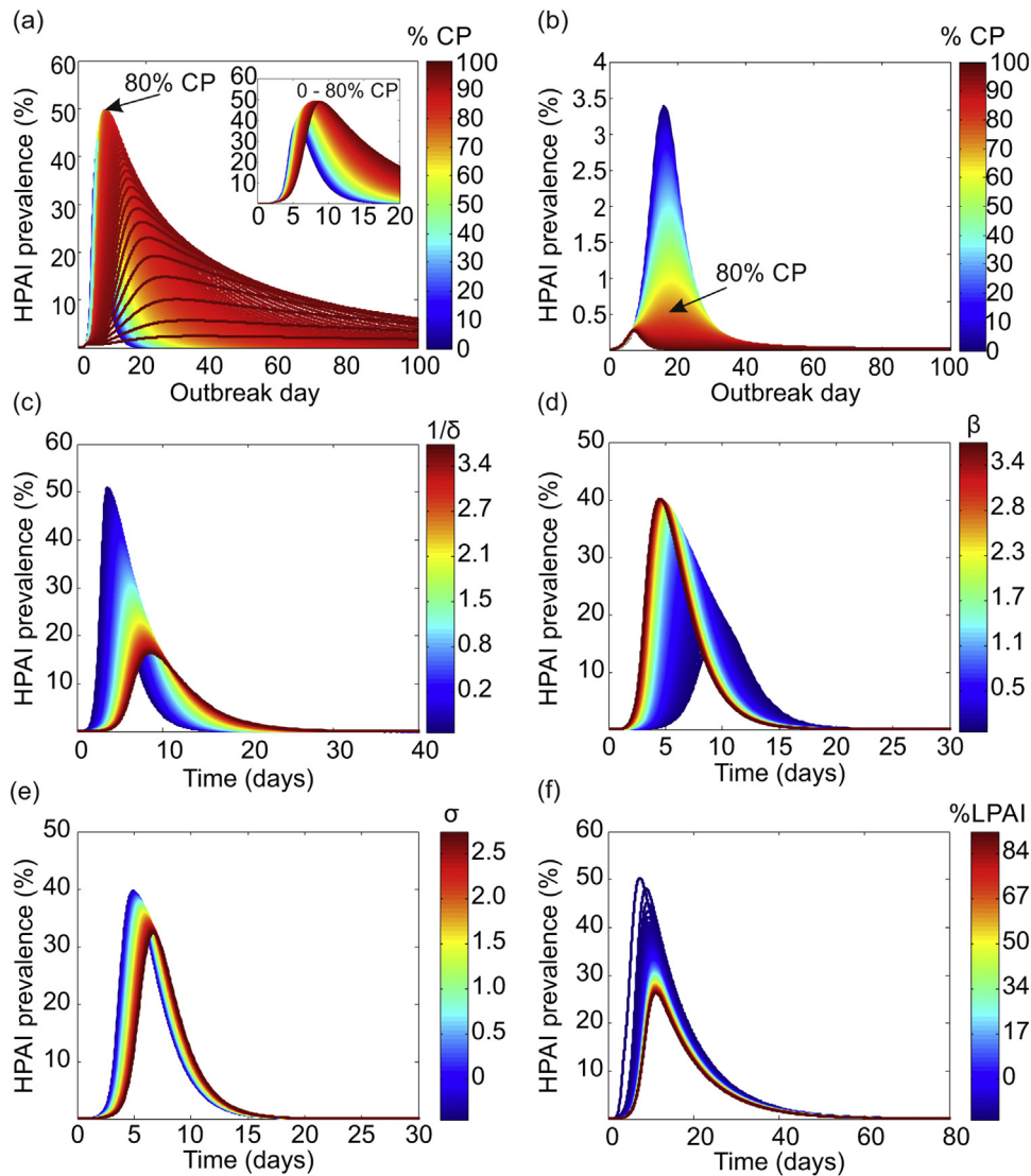
Fig. 2. Impact of immunological cross-protection on flock HPAI prevalence. Impact of immunological cross-protection (CP) on peak daily HPAI prevalence (% of birds infected with HPAI on a single day) assuming (a) aerosol and environmental transmission pathways. Inset shows results for 0%–80% CP, and (b) aerosol transmission only. Impact of varying levels of (c) HPAI infection latent period ( 1/\delta ), (d) HPAI transmission rate ( \beta ), and (e) HPAI environmental decay rate ( \sigma ) on peak daily HPAI prevalence under 0% CP, and (f) varying the background LPAI prevalence assuming 80% CP. See Table 1 for further details of the parameter values examined.
