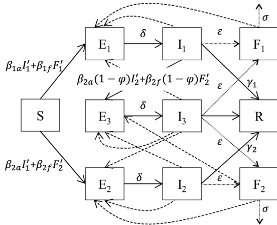
Fig. 1. Two-pathogen within-flock model schematic. Mechanistic model representing the co-circulatory dynamics of LPAI and HPAI transmission within a single densely populated commercial poultry flock. The proportions of birds in each infection class are denoted as follows: S = susceptible, E = exposed (but not yet infectious), I = infectious, R = removed (immune or dead). An additional F class represents the build-up of infectious faeces in the poultry house environment. Subscripts 1, 2 and 3 denote infection with LPAI, HPAI, and co-infection with both variants respectively. Solid arrows indicate the transition of birds from one infection state to the next. Dashed arrows indicate the contribution of birds in classes I and F to the forces of infection that generate newly infected birds. Dotted arrows in relation to F classes indicate the build-up (inward arrows) and decay (outwards arrows) of infectious faeces in the poultry house environment. Immunological cross-protection was incorporated through the assumed action of (i) reduced susceptibility of LPAI-infected birds to secondary HPAI infection, and (ii) increased survival of birds with secondary HPAI infection. See Table 1 for full details of the model parameters.
