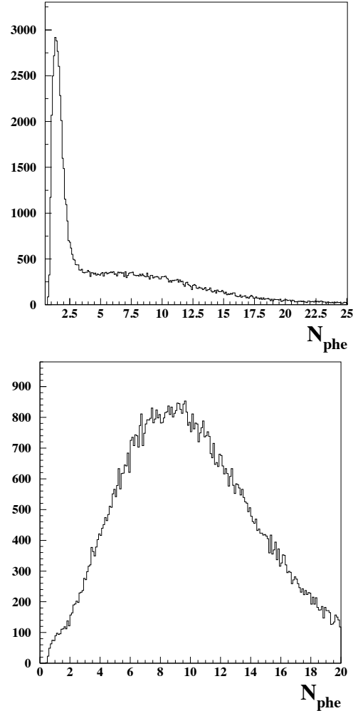
FIG. 9: Upper panel: The number of CC photoelectrons for events before the various cuts such as CC angle matching, EC sampling fraction and exclusivity cuts were applied. Lower panel: The number of CC photoelectrons for events that pass all cuts.
