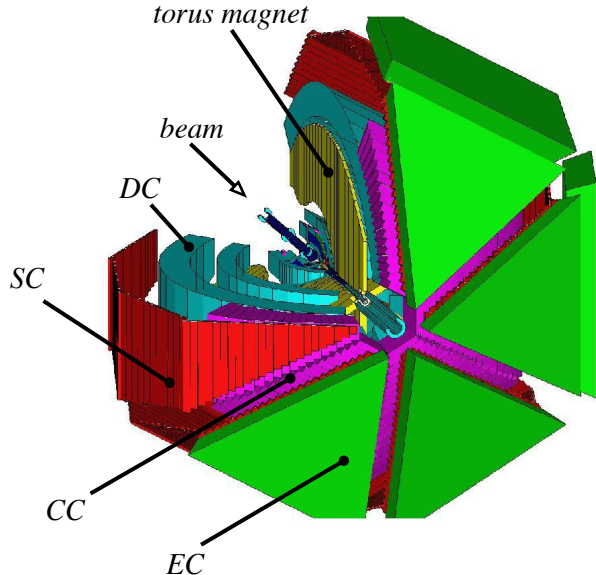
FIG. 3: (Color online) Three-dimensional schematic view of the elements of the CLAS detector with the different subsystems labeled. A single sector of the detector has been cut away to enable a view of the inner subsystems. The diameter of the CLAS detector is \sim 10 m. The notation is as follows: EC—Electromagnetic Calorimeter, CC—Cherenkov Counter, SC—Scintillation hodoscope, DC—Drift Chambers.
