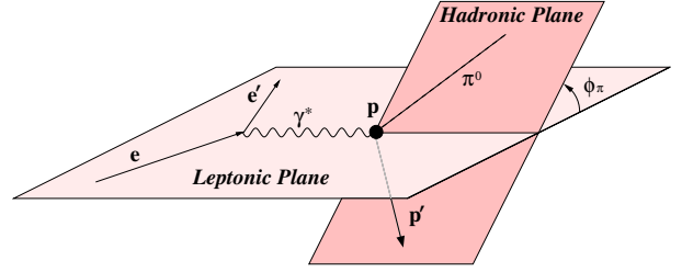
FIG. 25: The kinematics of \pi^0 electroproduction. \phi_\pi is the angle between the lepton and hadron planes. The lepton plane is defined by the incident and the scattered electron. The hadron plane is defined by the \pi^0 and the scattered proton.
