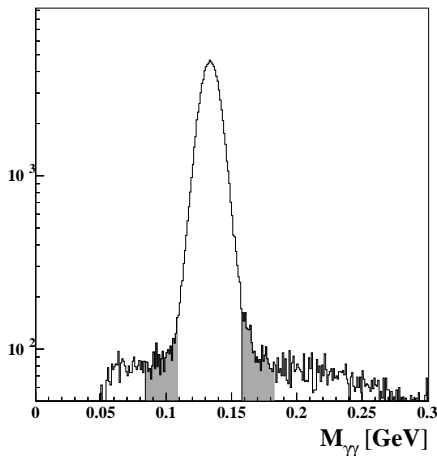
FIG. 12: The invariant mass distribution M(\gamma\gamma) for all events in which all selection criteria were applied, where both decay photons were detected in the IC (note the log scale). The shaded regions were used to estimate the residual background on a kinematic bin-by-bin basis.
