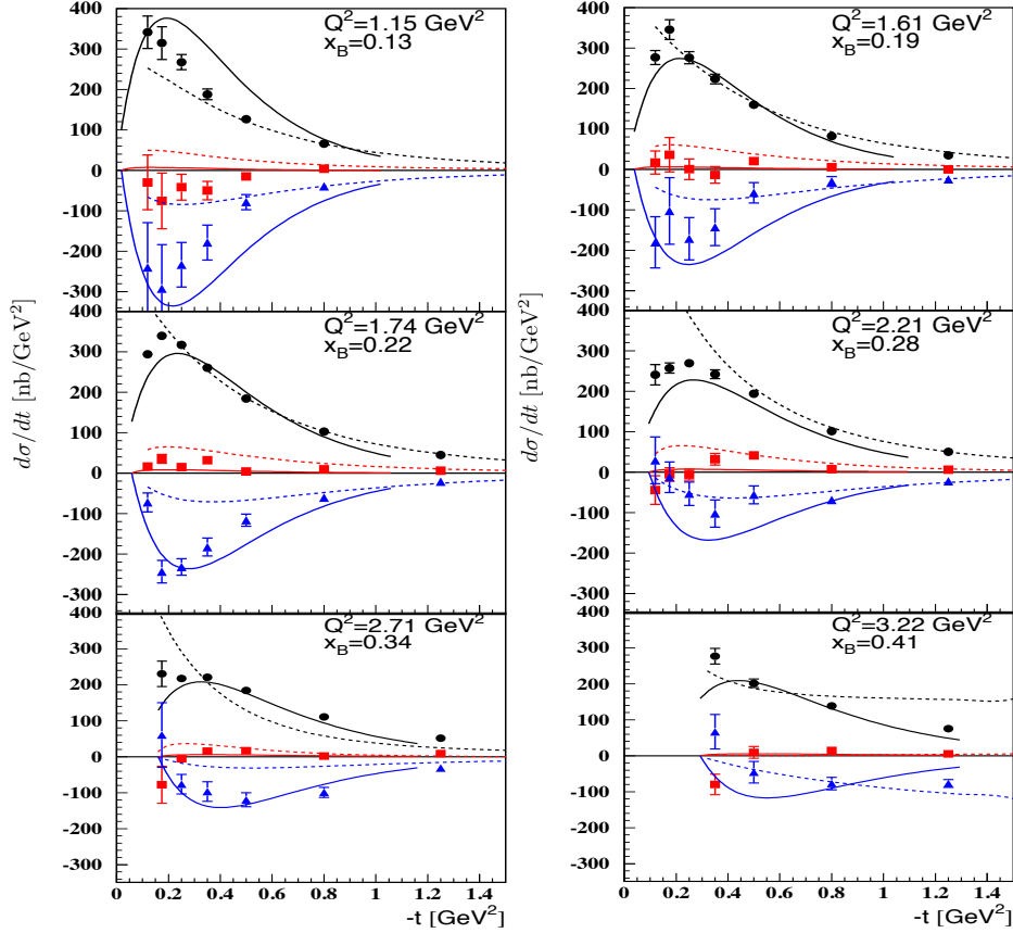
FIG. 23: (Color online) The extracted structure functions vs. t for the bins with the best kinematic coverage and for which there are theoretical calculations. The data and curves are as follows: black (filled circles) - d\sigma_U/dt = d\sigma_T/dt + \epsilon d\sigma_L/dt , blue (triangles) - d\sigma_{TT}/dt , and red (squares) - d\sigma_{LT}/dt . All the structure functions are numerically given in Appendix C. The error bars are statistical only. The point-by-point propagated systematic uncertainties for all the structure functions are given in Appendix C. The curves are theoretical predictions produced with the models of Refs. [33] (solid) and [19] (dashed). In particular: black (positive) - d\sigma_U/dt (= d\sigma_T/dt + \epsilon d\sigma_L/dt) , blue (negative) - d\sigma_{TT}/dt , and red (small) - d\sigma_{LT}/dt
