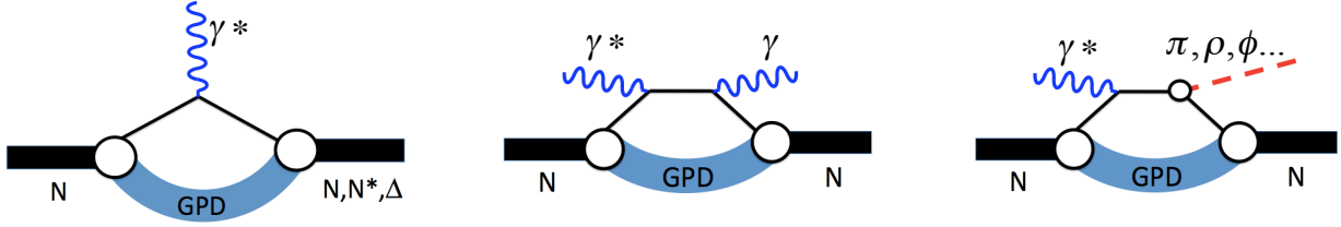
FIG. 1: Schematic diagram of the lowest order handbag mechanism applied to: (left) elastic scattering, (middle) DVCS and (right) meson production.
