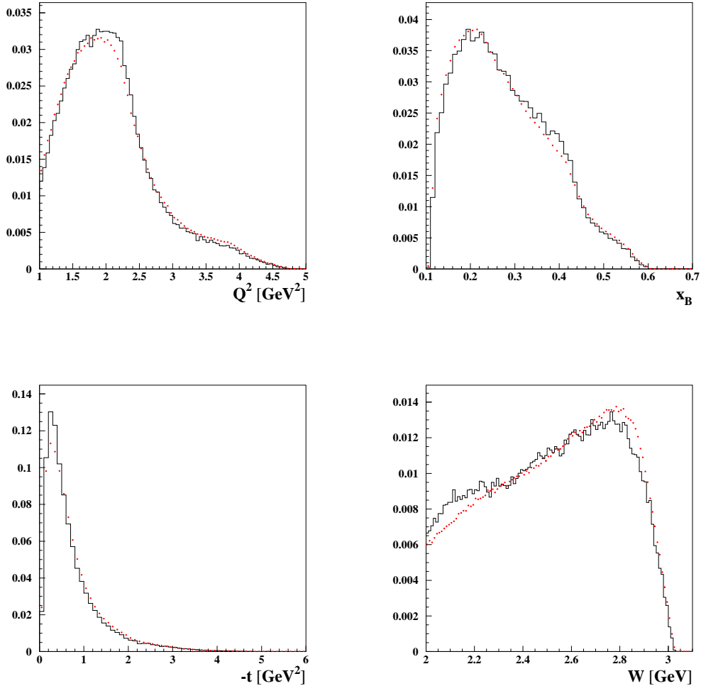
FIG. 7: (Color online) Distributions for kinematic variables Q^2 , x_B , -t and W in arbitrary units. The data are in black (solid) and the results of Monte Carlo simulations are in red (dotted). The areas under the curves are normalized to each other.
