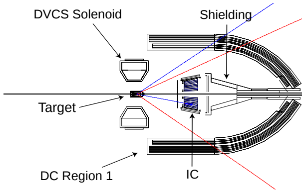
FIG. 5: (Color online) A blowup of Fig. 4 showing the CLAS target region in detail. IC is the inner calorimeter and DC-region 1 represents the drift chambers closest to the target.
