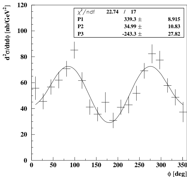
FIG. 19: Example of the \phi_\pi distribution of d^2\sigma/dtd\phi_\pi . The solid curve is a fit of the function in Eq. 9. The kinematic bin corresponding to this figure is at t = -0.18 \text{GeV}^2 , x_B = 0.22 and Q^2 = 1.75 \text{GeV}^2 and the data is listed in Table V. Error bars are statistical. The complete listing of all differential cross sections for all kinematic settings are found in Ref. [28].
