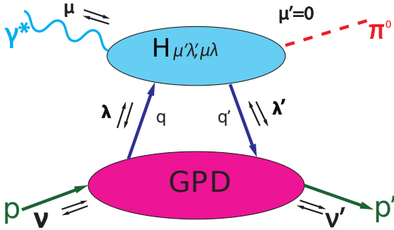
FIG. 2: Schematic diagram of the \pi^0 electroproduction amplitude in the framework of the handbag mechanism. The helicities of the initial and final nucleons are denoted by \nu and \nu' , of the incident photon and produced meson by \mu and \mu' and of the active initial and final quark by \lambda and \lambda' . The arrows in the figure schematically represent the corresponding positive and negative helicities, respectively. For final-state photons or vector mesons \mu' = \pm 1 , while for pseudoscalar mesons \mu' = 0 .
