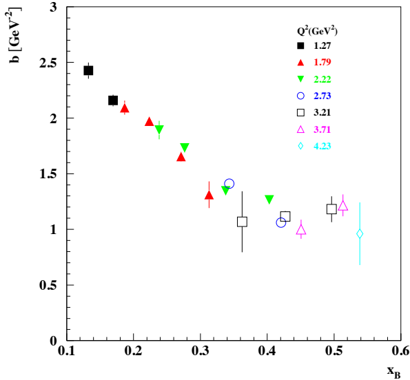
FIG. 18: (Color online) t -slope parameter b for the reaction \gamma^* p \rightarrow p' \pi^0 as a function of x_B for different values of Q^2 .
