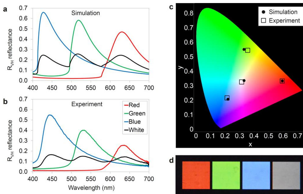
Figure 3. R_{VH} reflectance spectra and chromaticities for the RGB primary colours; simulations and experimental results. a , Simulations of the R_{VH} reflectance spectra at normal incidence for red, green and blue subpixel grating designs and their weighted combination in a white pixel. b , Experimental results showing the R_{VH} reflectance spectra for red, green, blue and white R_{VH} colour patches at normal incidence. c , The chromaticities of the R_{VH} primary colours and white pixel plotted on the CIE 1931 chart; simulations (circles) and experimental results (squares). d , An experimental result showing a calibrated image of the R_{VH} colour patches viewed through a V-H polarizing optical system (see Figure 4). Each patch measures 1.5 mm square. The white patch appears grey for the camera exposure used because each of the RGB patches is filled entirely with grating, whereas in an equivalent image pixel of those colours a maximum of approximately one third of the pixel area would be filled. Accordingly, the white patch is one third as bright as the corresponding RGB sum.
