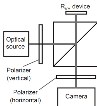
Figure 4. Schematic of the experimental setup for R_{VH} image recording.
