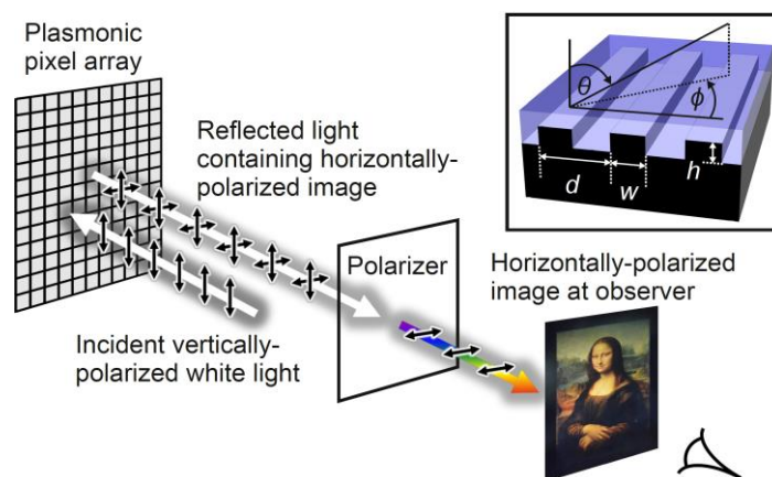
Figure 1. Concealed image generation using polarization conversion at a plasmonic pixel array. Schematic outlining the principles of image concealment and revelation. Inset: schematic of a portion of a metallic grating with a dielectric overlayer, indicating the polar angle \theta , the azimuth angle \phi with respect to the grating vector, the grating depth h , the pitch d and the ridge width w . The mark-pitch ratio r is given by w/d . The grating vector is orientated at 45^\circ to the vertical axis of the image.
