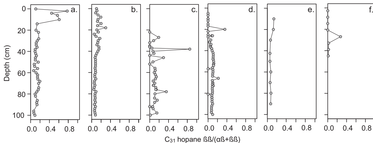
Fig. 3. Downcore C 31 hopane ββ/αβ + ββ profiles for Sphagnum -dominated peatlands. (a) Germany (Bissendorfer Moor), (b) Ireland (Ballyduff Bog), (c) Finland (Kontolanrahka Bog), (d) UK (Butternburn Flow), (e) Germany (Odersprung Bog), (f) Argentina (Tierra del Fuego).
