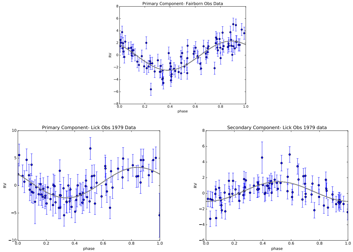
Figure A2. \delta Scuti pulsations in the residuals for the Fairborn and Lick RV data after the best fit orbit is subtracted out. The primary component of both datasets has a period of 0.157 days. The secondary in the Lick data has a period of 0.132 days. We detect no significant period signal for the secondary in the Fairborn Observatory data. Figures are phase-folded with T_0 = 56823.6 .
