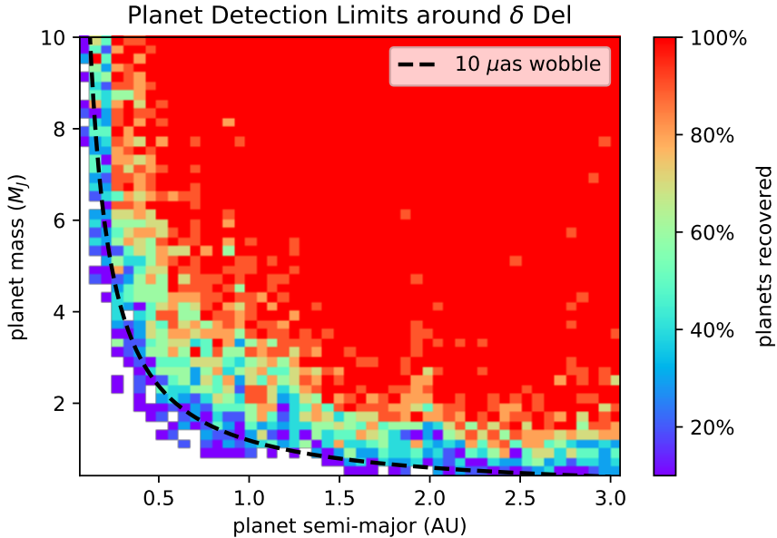
Figure 12. Planet detection limits around \delta Del are computed by simulating the wobble from a planet at each point on a mass, semi-major grid. A candidate detection is made based on the BIC criterion. If the best fit planet mass and semi-major axis are within 30% of the actual input values then we classify it as a true detection. For each mass, semi-major grid point we simulate 10 planets with random orbital elements and record the percentage of the time the planet is recovered. The dashed curve denotes the points on the grid where a planet would impart a 10 micro-arcsecond wobble on the star.
