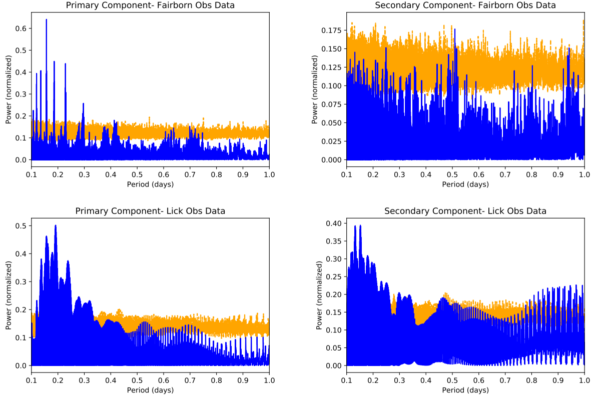
Figure A1. After subtracting out the best-fit RV orbit, we search for additional periodicity in the data due to \delta Scuti pulsations. We detect significant peaks in the primary component of the Fairborn data, and both components of the Lick data. The orange background signal depicts peaks of 3-sigma significance determined by bootstrapping. The peaks in the secondary component of the Fairborn data are not highly significant.
