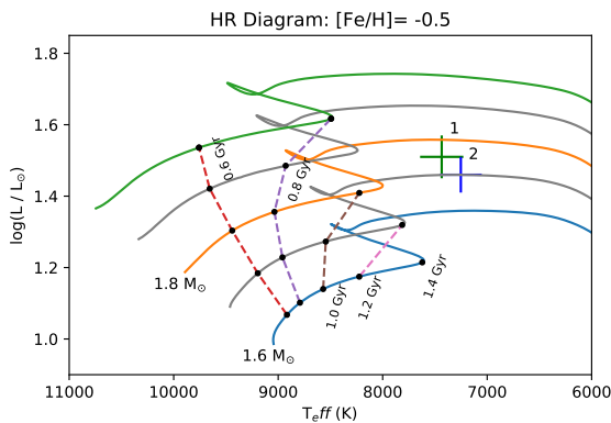
Figure 10. Position of both components of \delta Del on an HR diagram for the low metallicity case. MIST models are used to compute the plotted stellar tracks (solid lines) and isochrones (dashed lines). The luminosity and temperature values are consistent with our determined masses if component 2 is more evolved than component 1.
