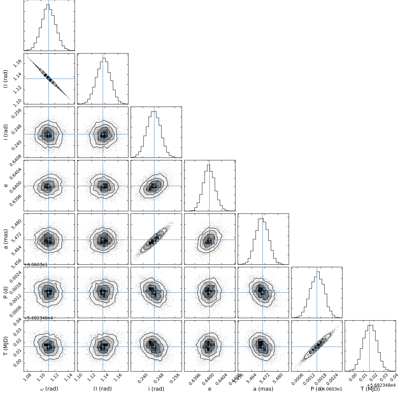
Figure 4. A corner plot of parameter distributions from the MCMC routine for astrometry data. Histograms display the number of times a given value was chosen as the best value for that element, and 2D plots show correlations between parameters. The crosshairs denote the best fit from least-squares fitting.
