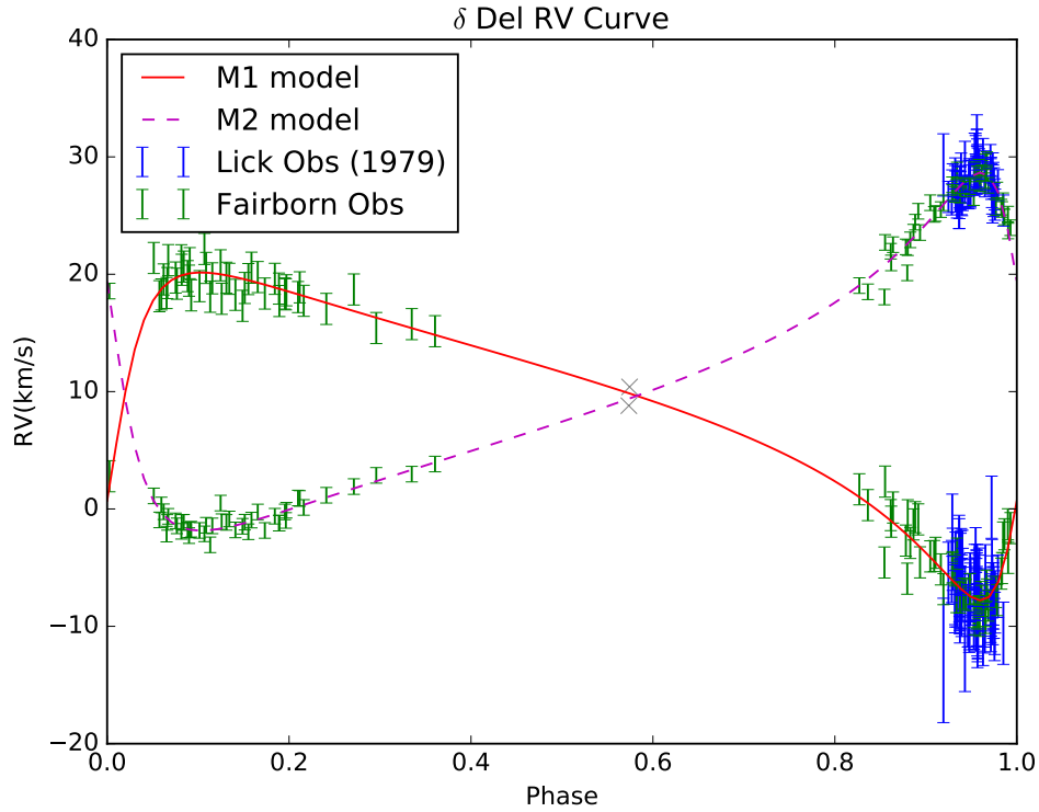
Figure 5. Double-lined radial velocities along with the best fit model. The RV data combines 97 data points from Fairborn Observatory with Duncan & Preston (1979)’s 87 unpublished RVs from Lick Observatory. The two gray marks just before phase 0.6 are velocities obtained from single-lined spectra. These points are not included in the best fit, but the measurements do help support our system velocity and mass ratio values.
