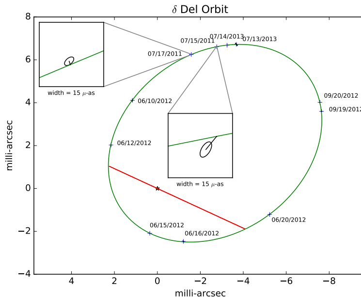
Figure 3. The position of the primary component relative to its companion at the origin. The green ellipse is the best fit orbit for \delta Del determined by fitting to astrometry data. The error ellipses on each observation are too small to be seen at this scale, so the insets display representative errors. The red line is the line of nodes, about which the orbit is inclined. Orbital motion is counterclockwise, with the portion of the orbit above the line of nodes inclined towards the observer and the portion below the line inclined away.
