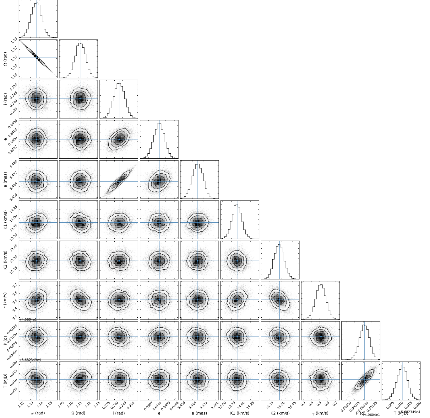
Figure 9. A corner plot of parameter distributions from the MCMC routine for combined astrometry and RV data. Histograms display the number of times a given value was chosen as the best value for that element, and 2D plots show correlations between parameters. The crosshairs denote the best fit from least-squares fitting.
