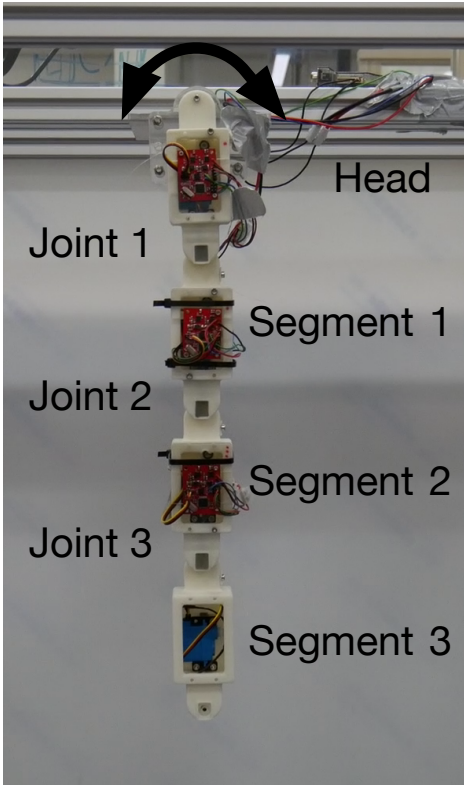
Fig. 2: The variable stiffness swimmer. The head is driven by a motor, while the remaining segments are passive. Joint stiffness is adjusted by a MACCEPA [26] inspired mechanism inside each segment.
