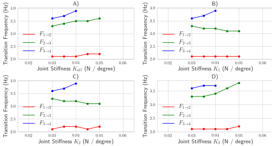
Fig. 9: Transition frequencies ( f_{1 \rightarrow 2} , f_{2 \rightarrow 3} , and f_{3 \rightarrow 4} ) against joint stiffness. A) shows the effect of increasing the stiffness of all joints simultaneously, while B), C), and D) show the effect of increasing the stiffness of joints 1, 2, and 3 separately.
