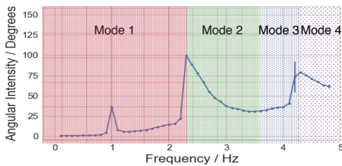
Fig. 7: Frequency response of the VSS in its most compliant state driven at an amplitude of 5 degrees. The plots show the tail beat intensity of the VSS as frequency is increased. Shaded areas indicate the different behavioural modes.
