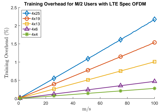
Fig. 5. The percentage of OFDM symbols that will be required to train M/2 (50) users at different speeds in the aforementioned LOS scenario. Array configurations of varying azimuth size considered using 10% decorrelation as a threshold for T_c , 300 kHz as a first order approximation of B_c and an LTE OFDM symbol duration of 71.4 \mu s
