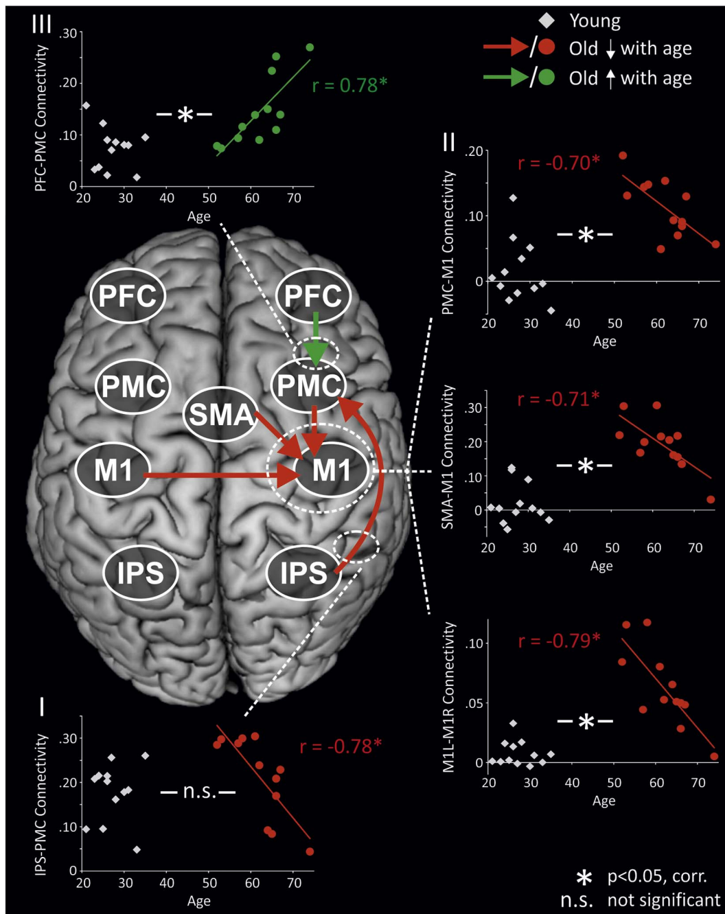
Fig. 4. Network changes with advancing age. Correlations between advancing age and coupling parameters (DCM-A) in old individuals. Coupling parameters of young subjects are indicated by grey diamonds and shown for illustrative purposes to underline between-group differences for the respective connections. Coupling parameters for older subjects are indicated by red circles for connections displaying a negative correlation with age, and by green circles for connections showing a positive correlation with age. Three different patterns of differential connectivity changes emerged: (I) IPS-PMC: no group difference between young and old subjects, negative correlation with age in old subjects. (II) Coupling targeting M1: enhanced connectivity in older individuals at the group level, negative correlation with age in older subjects. (III) PFC-PMC: enhanced connectivity in older individuals at the group level, positive correlation with age in older subjects. Note that all correlations shown remained significant when controlling for structural atrophy as informed by the VBM analysis. PFC = prefrontal cortex, PMC = premotor cortex, SMA = supplementary motor area, M1 = primary motor cortex, IPS = intraparietal sulcus. * p < 0.05, FDR-corrected for multiple comparisons; n.s. = not significant. Coupling strength in 1/s.
