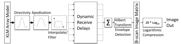
Fig. 6. MATLAB digital beamformer data flow. Data from the KLM model and acoustic phantom are stored in a matrix simulating the output from a full synthetic aperture scan and read into the beamforming algorithm in sets based on the programmed aperture size and step. The generated log-compressed image can be displayed as a linear image or can be subject to a Cartesian to polar conversion to display an anatomically correct image.
