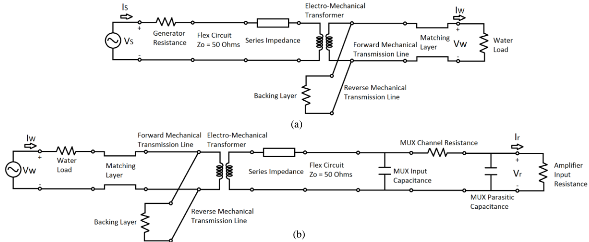
Fig. 2. Full KLM models for the a) tx and b) rx circuits. Voltage and current conventions for the KLM system definition have been labelled accordingly.
