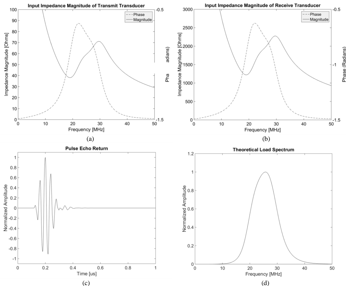
Fig. 7. KLM simulation results for the two-way tx-rx system. Input impedance magnitude for (a) tx and (b) rx transducers. The pulse-echo behaviour is shown in (c) the time- and (d) the frequency domains. The impedance magnitude is much larger for the rx transducer than for the tx transducer principally because the rx transducer has a much smaller surface area.
