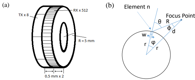
Fig. 4. Defined geometry for the curved array and the directivity. (a) The physical configuration of the tx and rx elements as simulated. (b) The effect of the curvature on the directivity calculation. Directivity values based on angle \theta are used in the calculation of both suitable rx apertures and the weighting functions for received acoustic echoes. As the tx pulses are unfocused, no directivity is assumed on transmission.
