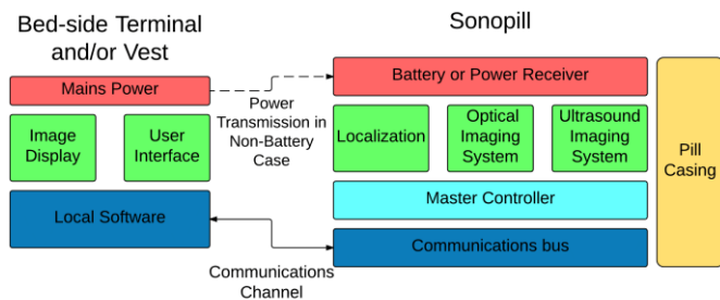
Fig. 1. System components and data flow for the proposed Sonopill capsule. Subsystems are colour-coded by function: red represents power; light blue represents integrated electronics; dark blue represents the system interface and communications; green represents key functional subsystems; and beige represents physical integration components.
