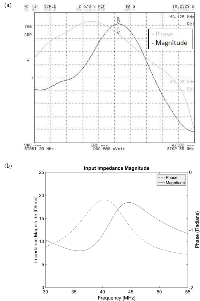
Fig. 3. Verification of KLM resonance calculations with experimental data, (a) measured impedance curve (magnitude and phase) of the transducer with anti-resonance marked, (b) corresponding simulation results with matching anti-resonance.
