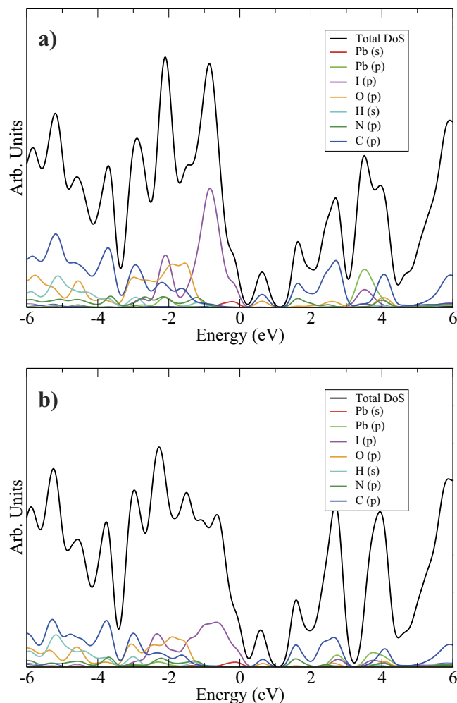
Figure 2. Total and Partial Density of States diagrams, using (a) PBEsol and (b) PBEsol + SOC; individual partial DoS are labelled in legends, Energy = 0 eV is set to valence band maximum and gaussian smearing of 0.2 eV was used.
