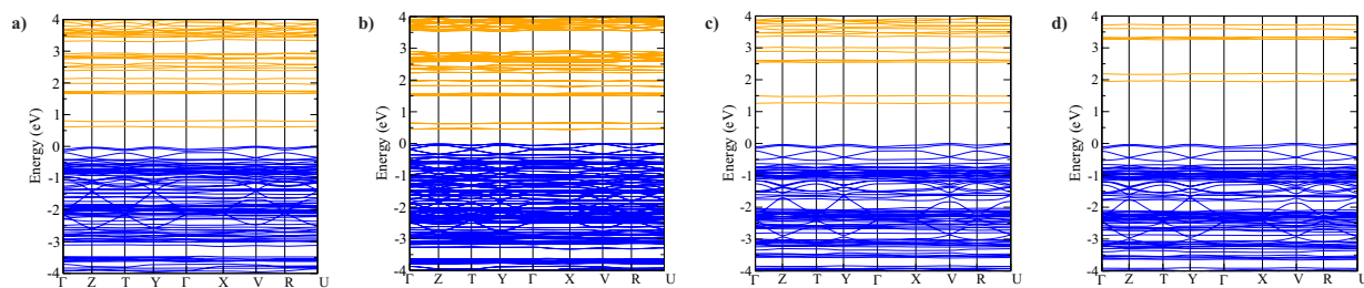
Figure 4. Band structure diagrams, using (a) PBEsol, (b) PBEsol + SOC, (c) HSE06, and (d) PBE0; valence band marked in blue, conduction band marked in orange, Energy = 0 eV is set to valence band maximum.
