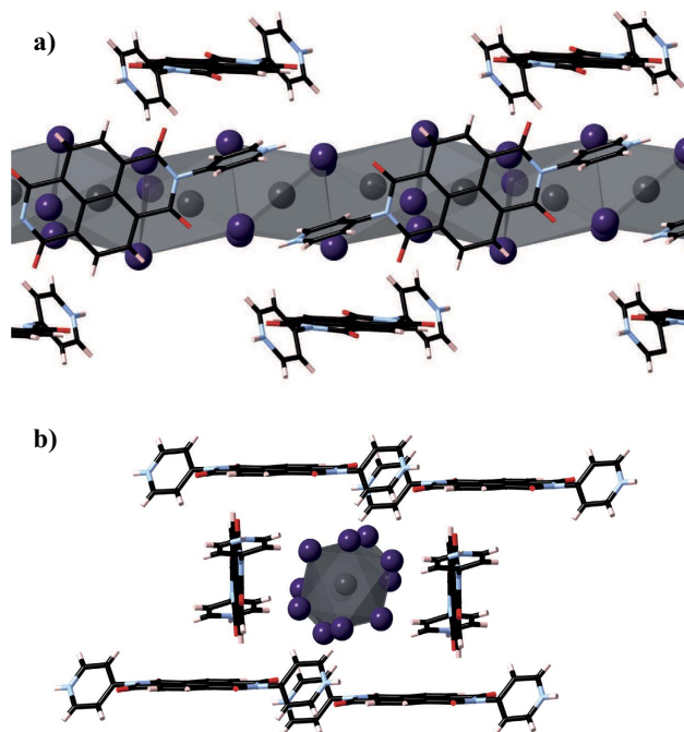
Figure 1. (\text{Pb}_2\text{I}_6) \cdot (\text{H}_2\text{DPNDI}) \cdot (\text{H}_2\text{O}) \cdot (\text{NMP}) , with solvent molecules removed for clarity and viewed along: (a) the a crystallographic axis, and (b) a single [\text{Pb}_2\text{I}_6]^{2-} nanowire, showing the DPNDI network. Carbon atoms are marked in black, hydrogen in pink, oxygen in red, nitrogen in blue, iodine in purple and lead in grey.
