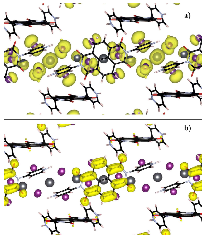
Figure 3. Plots of partial charge density at band edges: (a) Valence band; (b) Conduction band; viewed along the a crystallographic axis, with electron density marked in yellow.
