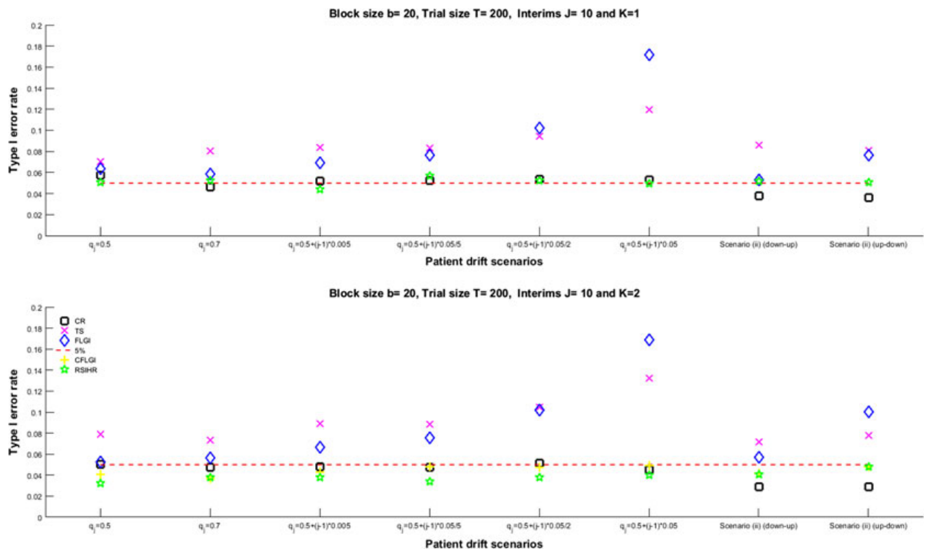
FIGURE 3 The type I error rate for different group recruitment rates assumptions under scenario 2 with \beta_z \approx 1.2528 . CR, complete randomisation; CFLGI, controlled forward-looking Gittins index rule; FLGI, forward-looking Gittins index rule; RSIHR, minimise failures given power; TS, Thompson sampling
