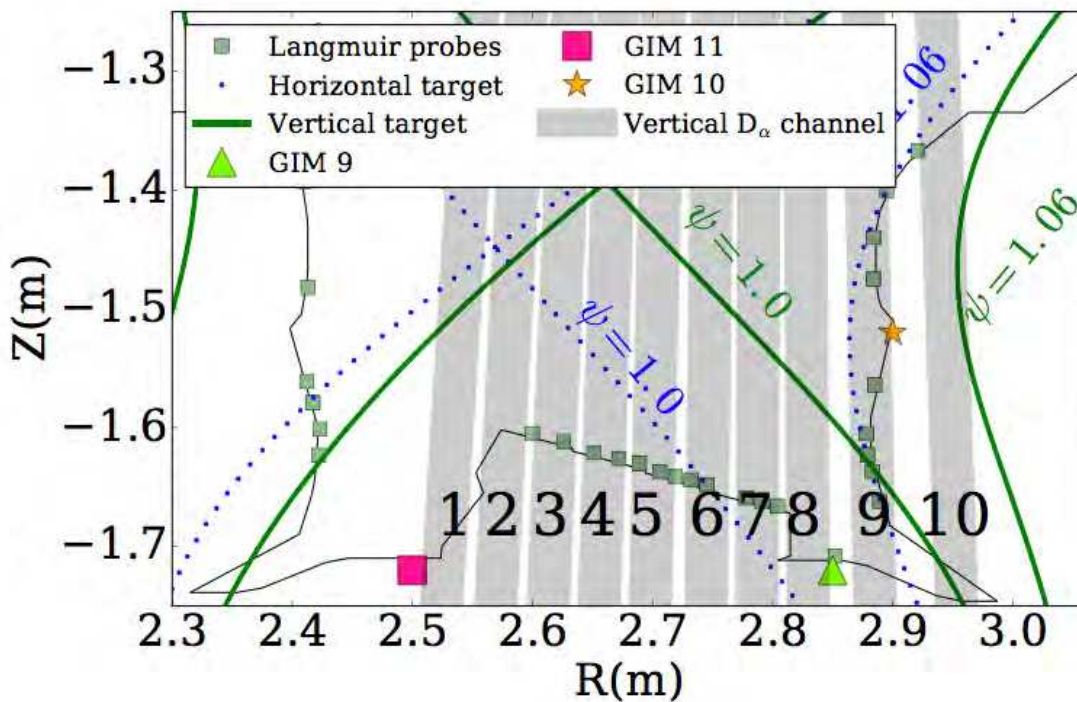
Figure 2: Close up of the divertor region of Fig. 1, showing the locations of the vertical viewing D_\alpha channels, Langmuir probes, Gas Injection Modules (GIMs) and the vertical and horizontal targets equilibria.
