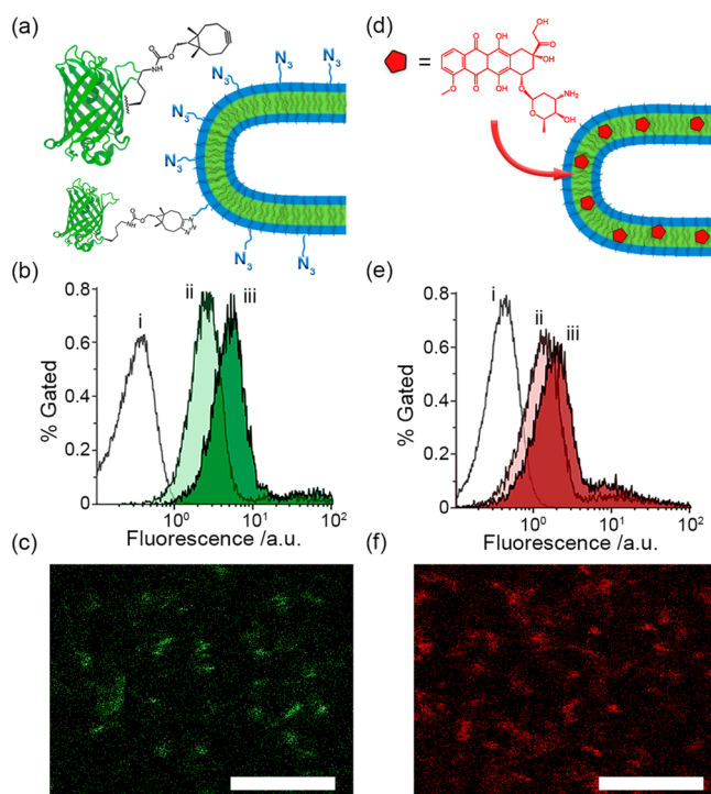
Figure 3. (a) Schematic outlining the covalent modification of azide-modified nanotubes using eGFP BCN , (b) flow cytometry data for eGFP BCN modification of 5% azido nanotubes using an equimolar (ii) or a 3-fold excess (iii) of eGFP BCN compared to unmodified tubes (i) and (c) confocal visualization of green-fluorescent nanotubes. (d) Schematic outlining the loading of nanotubes with fluorescent DOX, (e) flow cytometry data of nanotubes loaded with 2 (ii) and 5 (iii) wt % DOX compared to unloaded tubes (i) and (f) confocal visualization of DOX-loaded nanotubes (5 wt % preparation). All scale bars = 5 μm.
