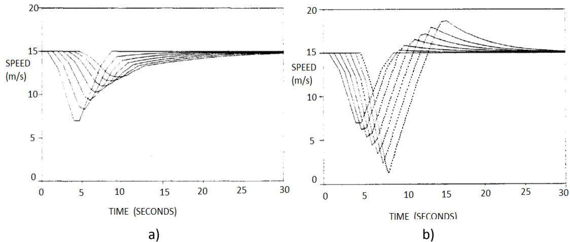
Figure 9. Speed-time plots for seven successive vehicles using Gipps' model with following parameters: \mathbf{a_n = 2 \frac{m}{s^2}, b_n = -3 \frac{m}{s^2}, v_n = 30 \frac{m}{s}} and \boldsymbol{\tau = \frac{2}{3} \text{ sec}} when a) \hat{\mathbf{b}} = -3.5 \frac{m}{s^2} b) \hat{\mathbf{b}} = -2.5 \frac{m}{s^2} [38].
