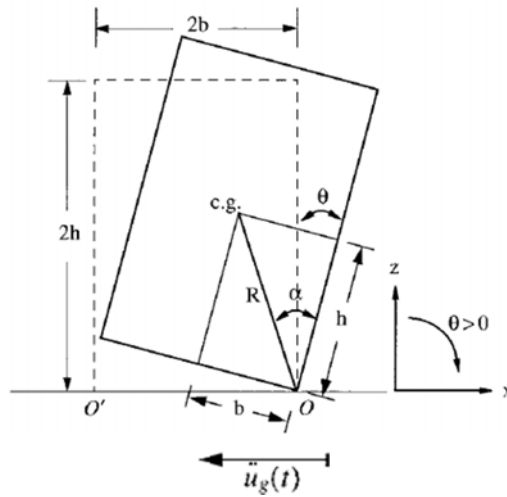
Figure 1. Free-standing rigid block.
