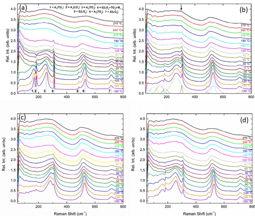
Fig. 7 In-situ Raman spectroscopy for (a) undoped BaTiO 3 , (b) 1 mol% doped BiYbO 3 , (c) 2 mol% doped BiYbO 3 and (d) 1 mol% doped LaYbO 3 .
