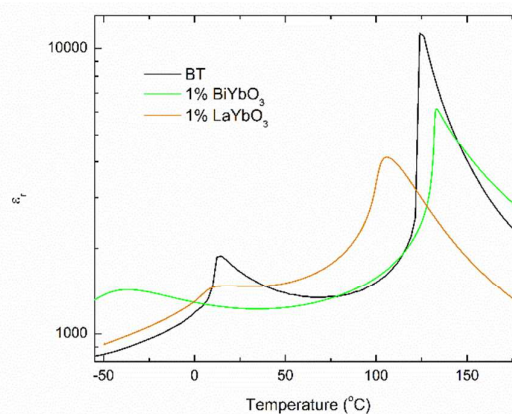
Fig. 6 Temperature dependence of the relative permittivity for (1-x)\text{BaTiO}_3-x\text{BiYbO}_3 and (1-x)\text{BaTiO}_3-x\text{LaYbO}_3 ceramics in the 0 \leq x \leq 0.01 range.
