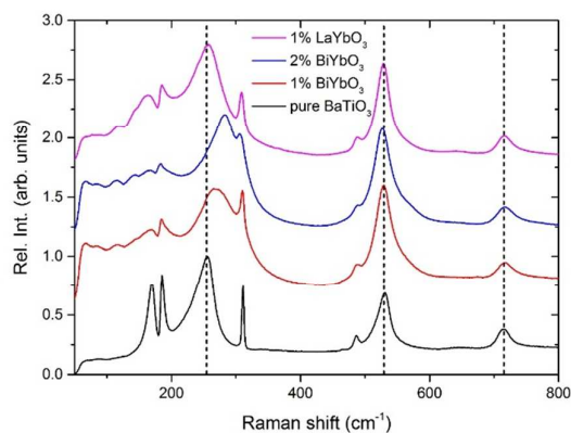
Fig. 9 Composition-dependent Raman spectra of BiYbO 3 and LaYbO 3 -doped barium titanate at -180°C.
