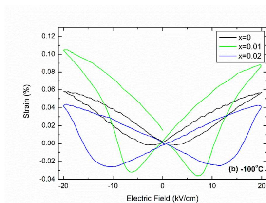
Fig. 4 Electric-field induced strain at (a) 50 °C and (b) -100 °C for (1-x)\text{BaTiO}_3-x\text{BiYbO}_3 ceramics.
