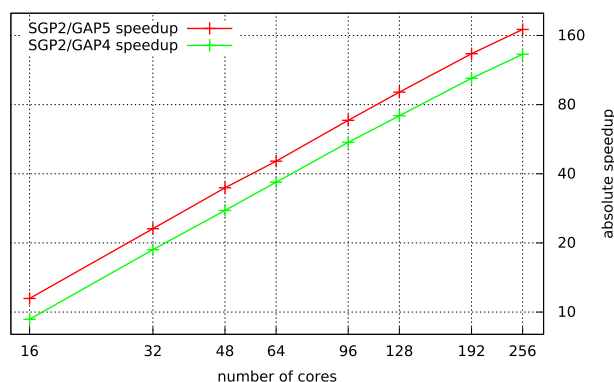
Figure 15. SGP2 with GAP4 and GAP5 SumEuler speedups (Beowulf).
