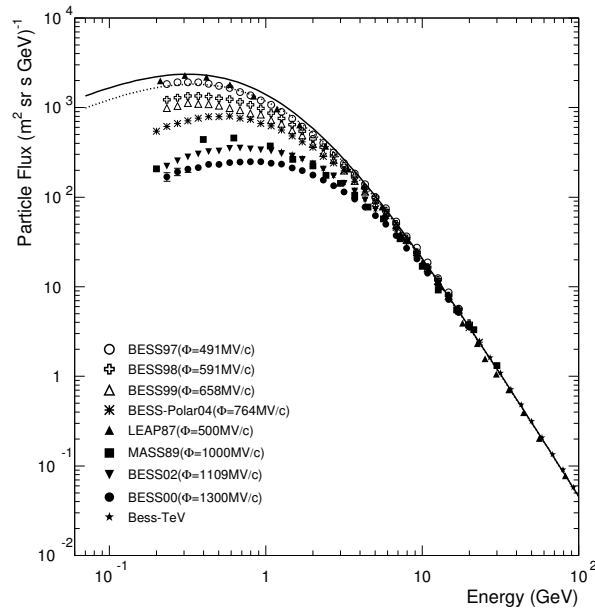
Figure 10. GCR proton energy spectra measurements and projections before (continuous line) and at the deep (dotted line) of the depression observed on August 2, 2016 with LPF.
