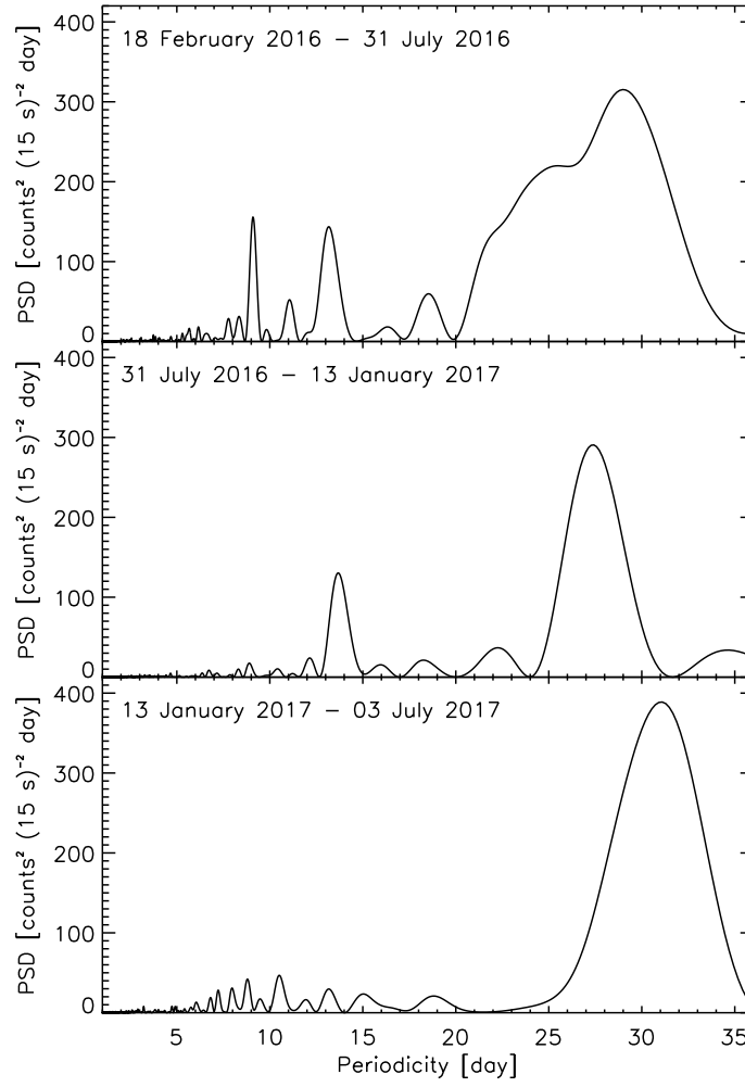
Figure 5. Power spectral density from the Lomb-Scargle periodogram analysis applied to the PD data gathered in the time interval indicated in each panel (which refers to one third of the whole LPF PD data set). Sun rotation and higher harmonics periodicities are modulated throughout the observational period.
