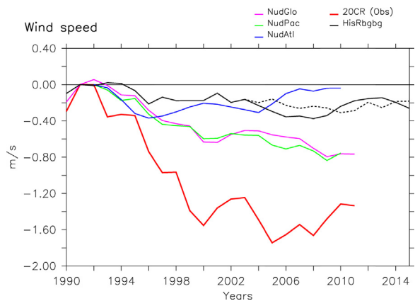
Fig. 6. Wind velocity in the western tropical Pacific (6°S–6°N, 150°W–180°W, cf. Fig. 5a) in the different simulations, following the box definition from England et al. (2014). A 5-year running mean has been applied on all time series, and they have been centered over the mean of the years 1990–1994.
