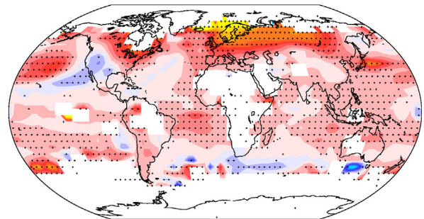
Fig. 4. Spatial map of surface temperature trend (in 0.1\text{ }^{\circ}\text{C}/\text{yr} ) over the period 1998–2012. The significant trends following a two-sided student test are stippled in black. (a) HadCRUT4 data, (b) NudGlo ensemble mean, (c) NudPac ensemble mean, (d) NudAtl ensemble mean, (e) HisRnobg ensemble, and (f) HisRbg ensemble mean.
