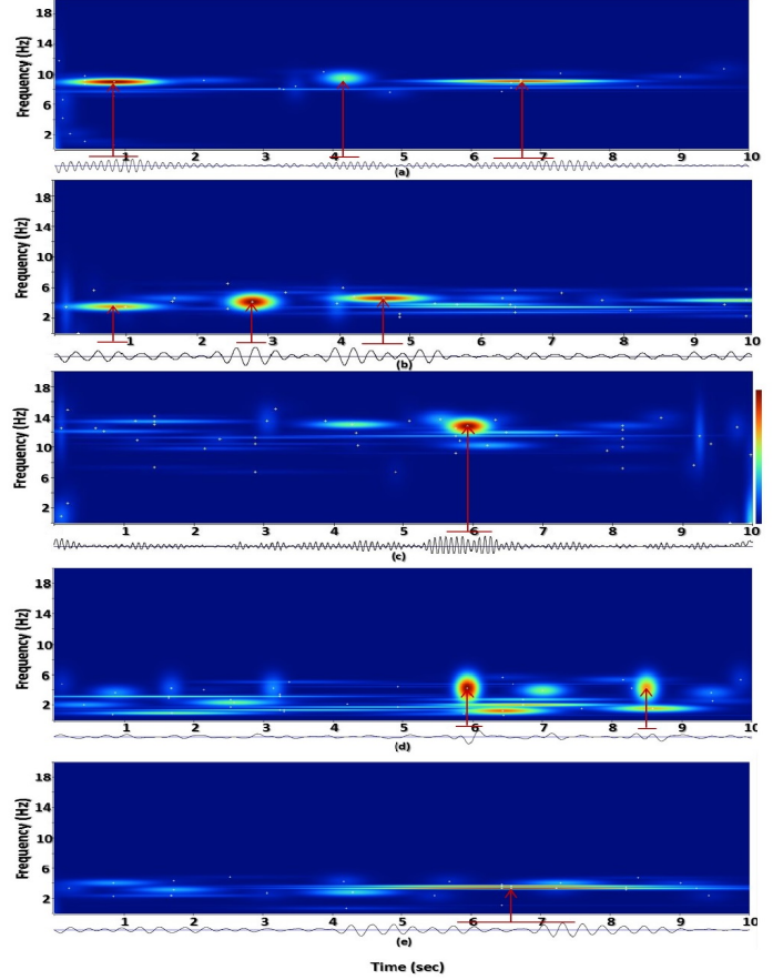
Figure 3: T-F representation of different sleep EEG stages of the same subject as in Figure 2 using the proposed constrained SSA; (a) awake, marked alpha; (b) N1, marked theta; (c) N2, spindle; (d) N2 K-complex; and (e) SWS.
