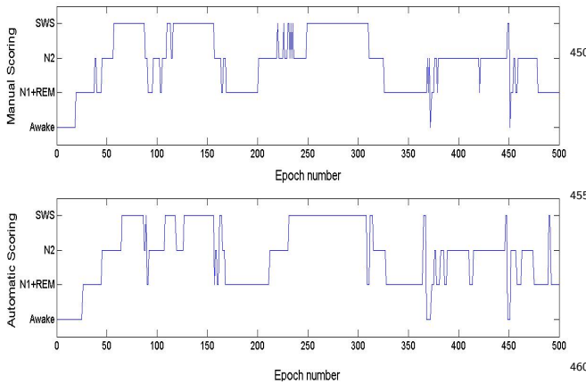
Figure 6: Representative four sleep stage classification of 500 epochs acquired using clinical expert (top) and SSA (bottom).
