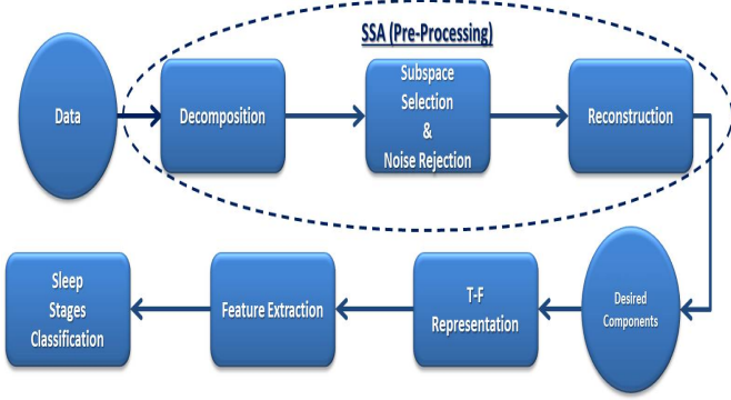
Figure 1: Block diagram of the proposed sleep scoring approach.
