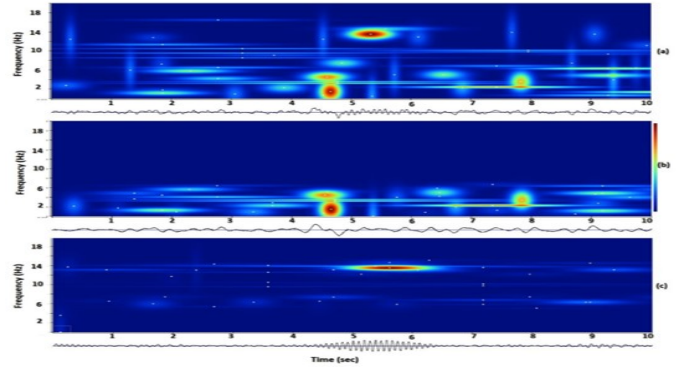
Figure 5: T-F representation of EEG signals of Figure 4; (a) original signal, (b) the extracted k-complex, (c) the extracted sleep spindle
