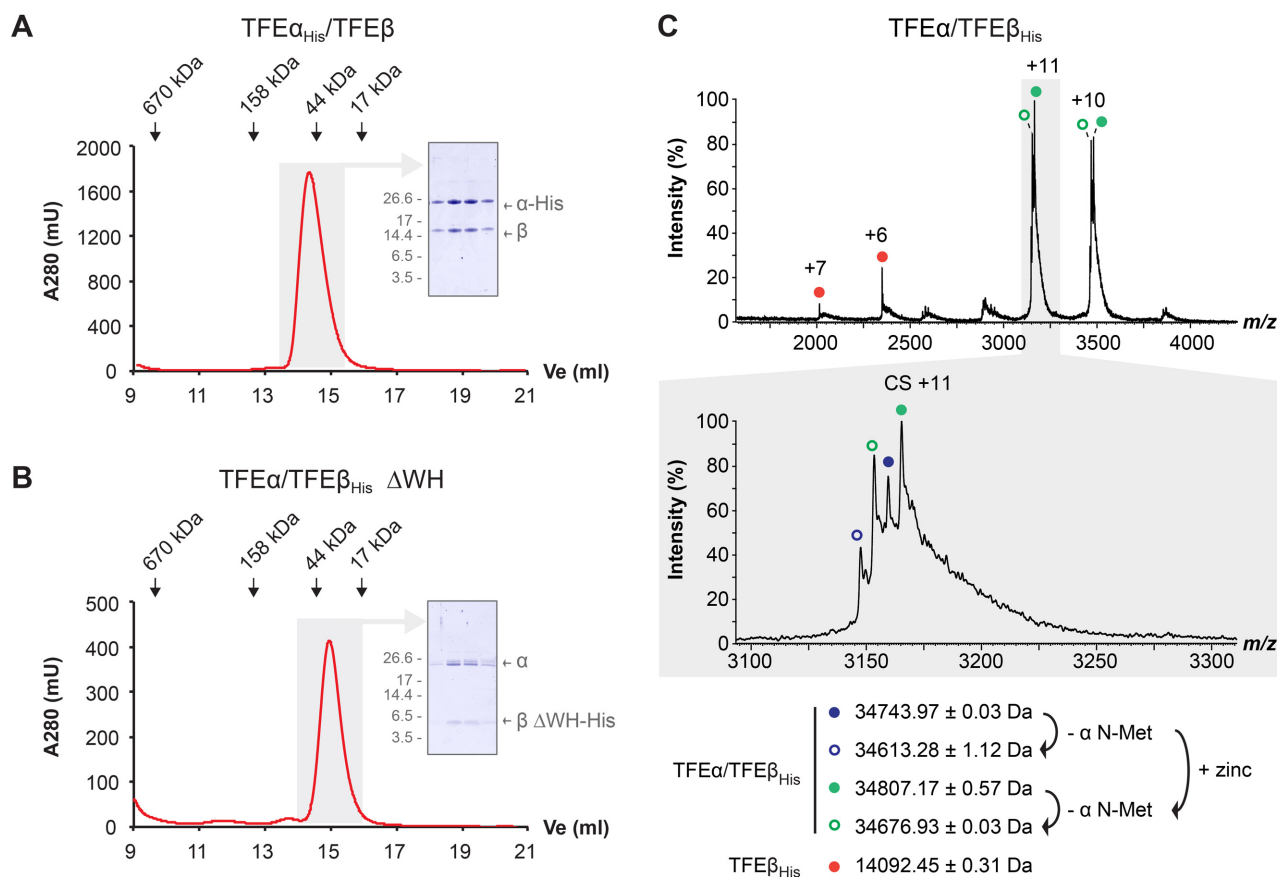
Figure 2. Hvo TFE \alpha and TFE \beta form a dimeric complex in the absence of an FeS cluster. (A and B) Size exclusion chromatography of TFE \alpha_{\text{His}} /TFE \beta (A) and TFE \alpha /TFE \beta \Delta WH \text{His} (B) on a superose 12 h 10/30 column. Elution peaks of standard proteins are indicated. Peak fractions (highlighted in gray) were subjected to SDS-PAGE and Coomassie-staining (insert) to show symmetric elution of both subunits. (C) nESI mass spectrum of TFE \alpha /TFE \beta_{\text{His}} . The different charge state series observed are labelled with red, blue and green filled circles. Charge state series derived from additional cleavage of TFE \alpha N-Met are labelled with open circles. Highlighted in gray is a zoom over the region that includes charge state (CS) +11. All detected masses indicate the absence of a cubane 4Fe-4S cluster (352 Da).
