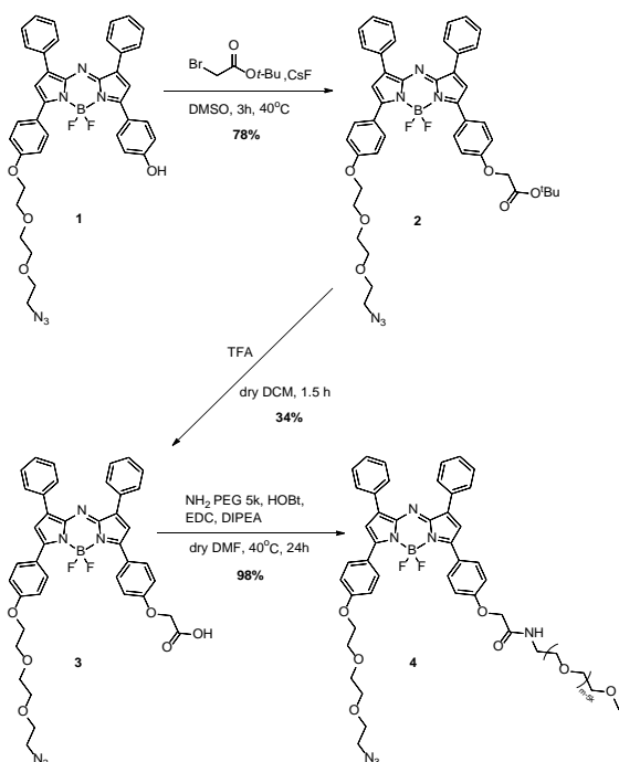
Scheme 1. Synthesis of water soluble azido aza-BODIPY.
