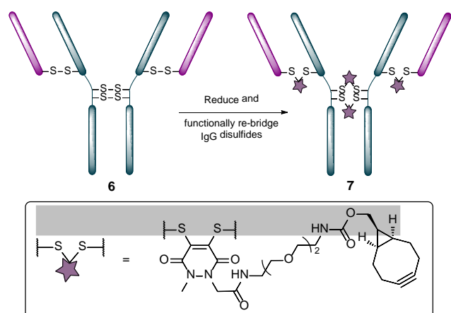
Scheme 2. Preparation of "clickable" trastuzumab 7 .
