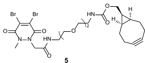
Figure 2. Structure of PD-based re-bridging reagent.
