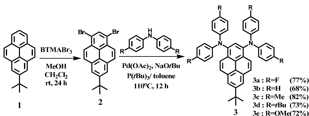
Scheme 1. Synthesis of pyrene-based light-emitting monomers 3 .
