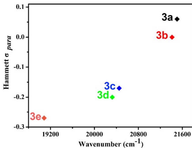
Figure 5. Hammett \sigma_{para} constants versus wavenumber (cm -1 ) for 3a (black), 3b (red), 3c (blue), 3d (green), and 3e (orange).
