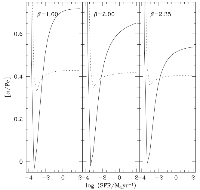
Figure 4. [\alpha/\text{Fe}] (solid lines) and [\text{Si}/\text{Fe}] (dotted lines) ratios as a function of the galaxy SFR, for different values of \beta (indicated on the top of each panel). We assume in this plot the reference value \hat{y}_{\text{Fe}} = 0 .
