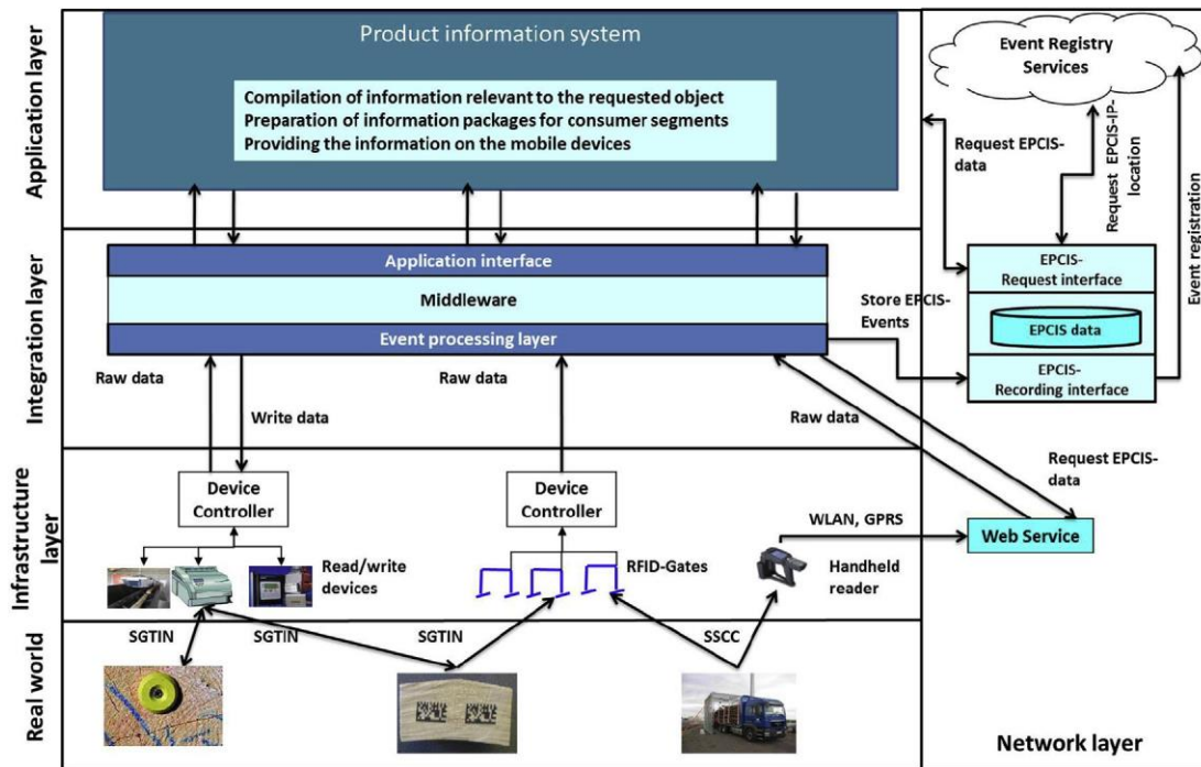
Fig. 7. System architecture (according to Thoroe et al., 2011).
