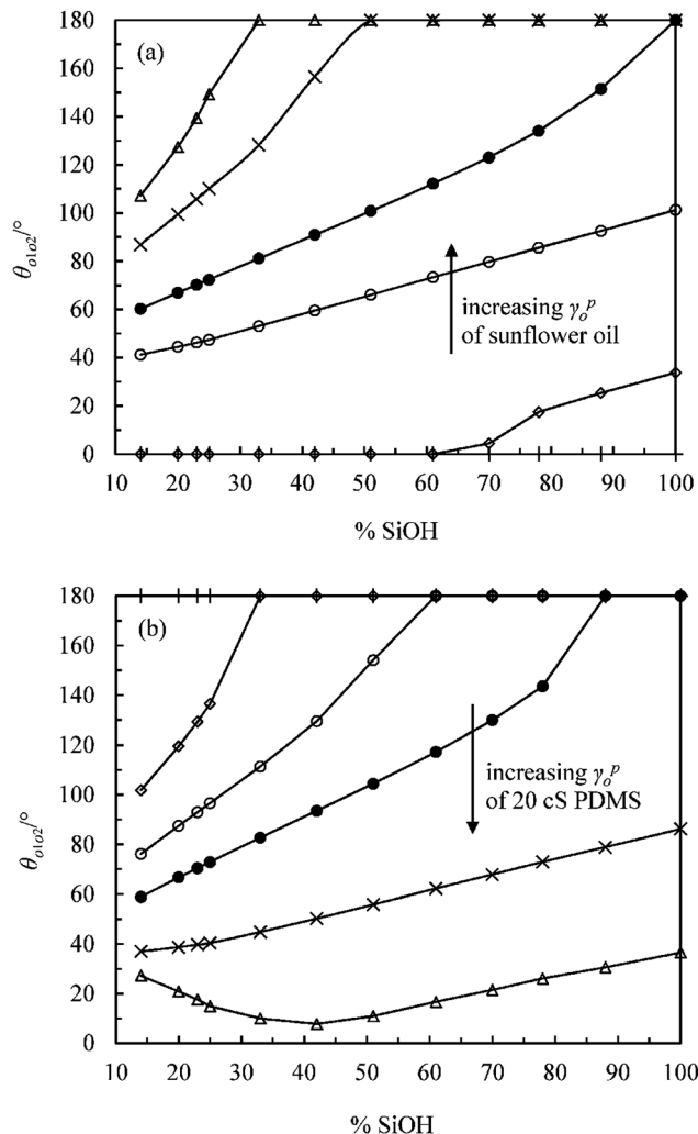
Fig. 8 Plot of calculated \theta_{\text{o}_1\text{o}_2} into PDMS versus % SiOH on DCDMS-coated silica particle surfaces for the interface sunflower oil-20 cS PDMS with (a) \gamma_{\text{o}}^{\text{p}} ; \gamma_{\text{o}}^{\text{d}} = 0 ; 33.3 (+), 0.2; 33.1 (◊), 0.4; 32.9 (○), 0.6; 32.7 (●), 1.0; 32.3 (×) and 1.4; 31.9 (Δ) \text{mN m}^{-1} for sunflower oil and \gamma_{\text{o}}^{\text{p}} ; \gamma_{\text{o}}^{\text{d}} = 0.9 ; 19.9 \text{mN m}^{-1} for PDMS and (b) \gamma_{\text{o}}^{\text{p}} ; \gamma_{\text{o}}^{\text{d}} = 0 ; 20.8 (+), 0.2; 20.6 (◊), 0.4; 20.4 (○), 0.6; 20.2 (●), 1.0; 19.8 (×) and 1.4; 19.4 (Δ) \text{mN m}^{-1} for PDMS and \gamma_{\text{o}}^{\text{p}} ; \gamma_{\text{o}}^{\text{d}} = 0.4 ; 32.9 \text{mN m}^{-1} for sunflower oil.
