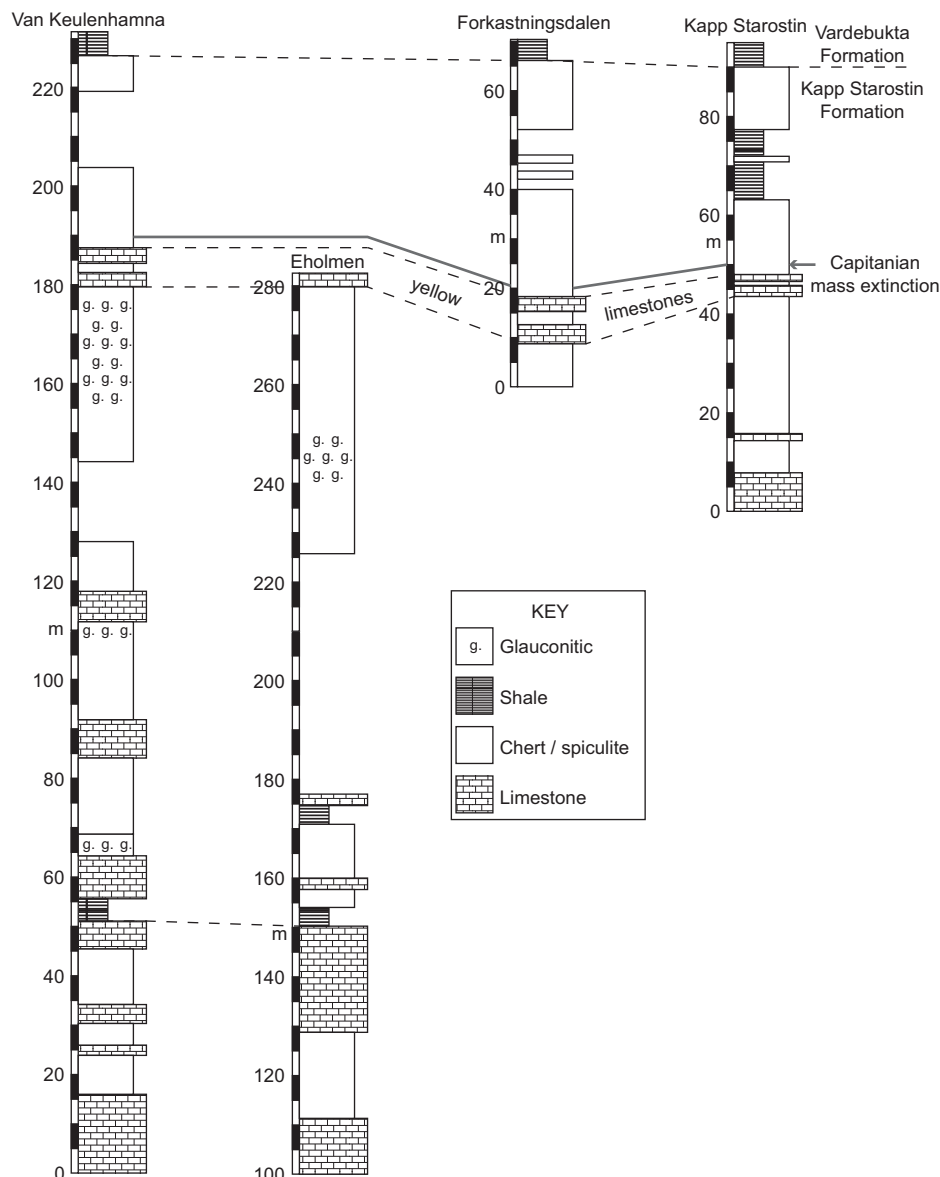
Figure 4. Correlation panel with simplified lithologic logs from Kapp Starostin (78.0950°N, 13.8240°E [WGS84 datum]), Van Keulehamna (77.6102°N, 14.9706°E [WGS84]), Eholmen (77.5982°N, 14.9146°E [WGS84]), and Forkastningsdalen (77.6427°N, 14.9041°E [WGS84]). The three yellow limestone beds (3YLB) that immediately precede the extinction horizon have been used to correlate between sections.
