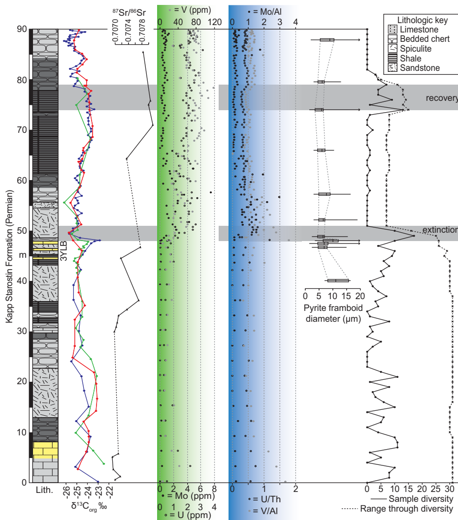
Figure 3. Log of the Kapp Starostin section (78.0950°N, 13.8240°E [WGS84 datum]) showing the upper part of the Kapp Starostin Formation up to the contact with the overlying Vardebukta Formation at 90 m height. Colors in the lithology column indicate pale gray, dark gray, and yellow beds (3YLB—three yellow limestone beds used for correlation between sections). Three separate organic carbon isotope ( \delta^{13}\text{C}_{\text{org}} ) curves were generated by M. Joachimski (red circles), Y. Sun (green circles), and S. Grasby (blue circles). All three curves are in excellent accord. The ^{87}\text{Sr}/^{86}\text{Sr} curve (black triangles) was generated from brachiopod shells: Low values in the lower part of the section are consistent with the Middle Permian low point of the global curve (Korte et al., 2006; see Fig. 1). The marked increase to more radiogenic values in the postextinction interval is suggestive of a Late Permian age for the upper part of the section, although the extremely high values in the topmost part of the section suggest diagenetic overprinting. Elemental concentrations of trace metals (green shaded box) show an enrichment in molybdenum (Mo, black circles), uranium (U, open circles), and vanadium (V, gray circles) in the extinction interval, suggesting anoxic conditions developed at Kapp Starostin in the Middle to Late Permian. Normalized trace metal analyses (blue shaded box) (Mo/Al, U/Th, V/Al) suggest that the enrichment in redox-sensitive metals is independent of facies/terrigenous input. Pyrite framboid box and whisker plots show the 25th and 75th percentiles of framboid diameters in each sample (horizontal extent of black box), mean framboid diameter (central vertical line), and maximum and minimum framboid diameter (long horizontal line). The diversity curve (diversity taken from the composite log in Fig. 7) depicts the number of brachiopod and bivalve taxa (circles and solid line). Range-through (standing) diversity (including taxa known to be extant at each level) is shown as crosses and dashed line. Mass extinction and recovery intervals are shaded gray.
